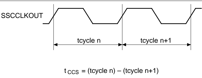
Figure 1 Cycle to cycle jitter (SSCCLKOUT)
