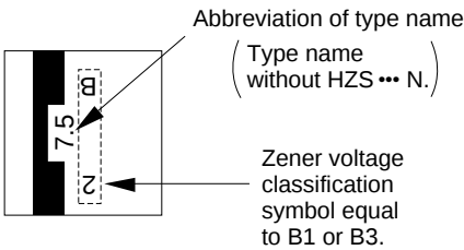
Expanded drawing of marking
