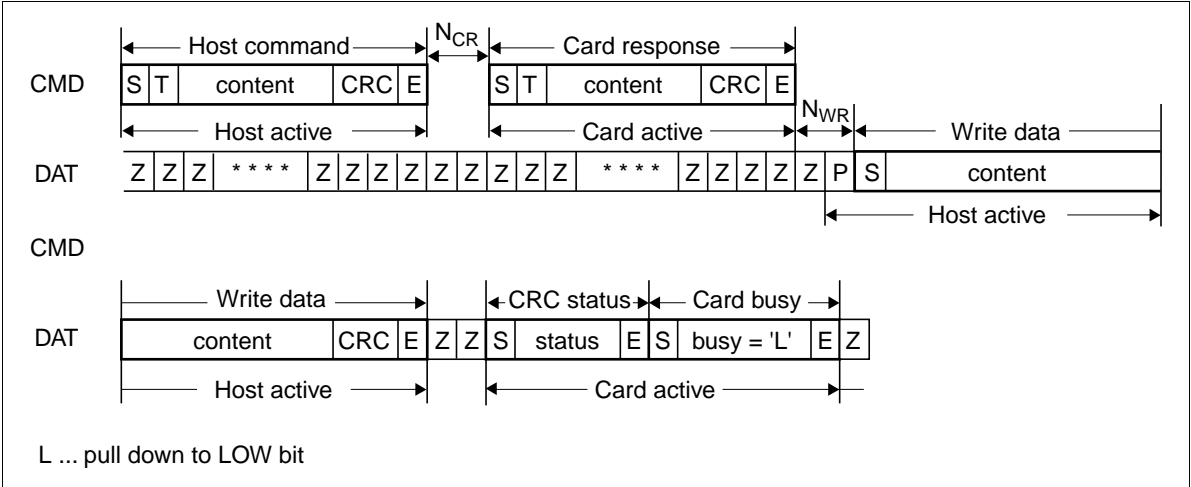
Timing of The Block Write Command
