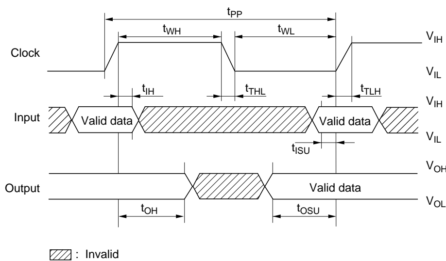
Timing Diagram of Data Input and Output
