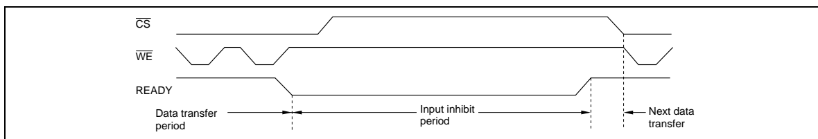
Figure 12 READY Output Timing (When It Is Always Available)
