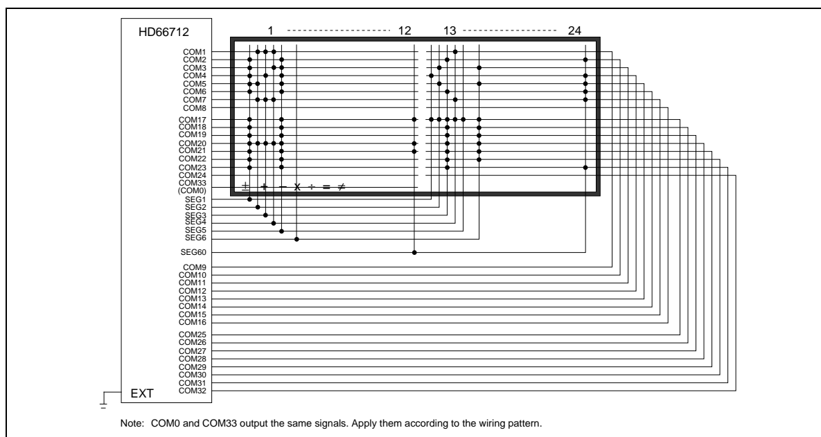
Figure 26 24 × 1-Line + 60-Segment Display (5-Dot Font, 1/33 Duty)
