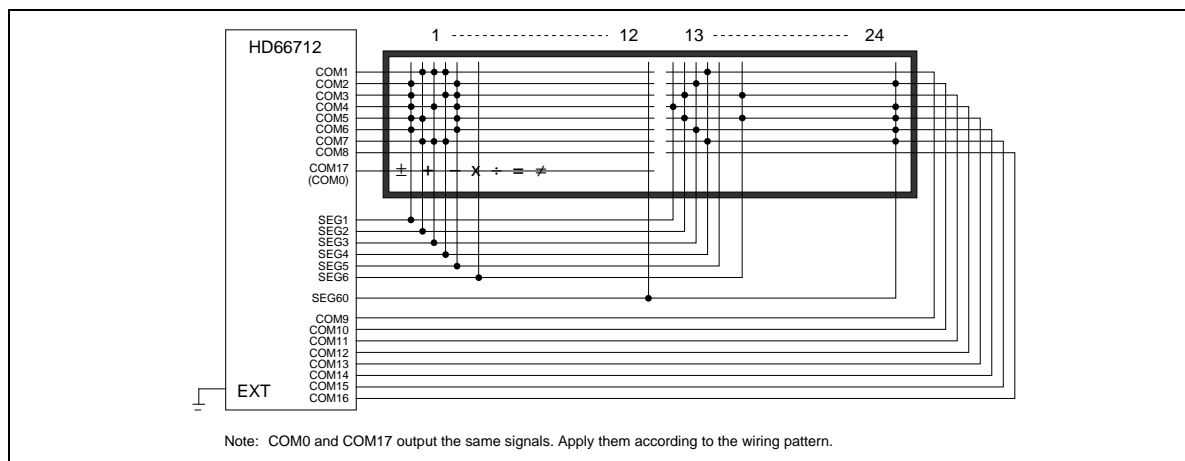
Figure 25 24 × 1-Line + 60-Segment Display (5-Dot Font, 1/17 Duty)
