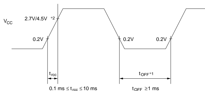
Figure 38 Reset Timing
