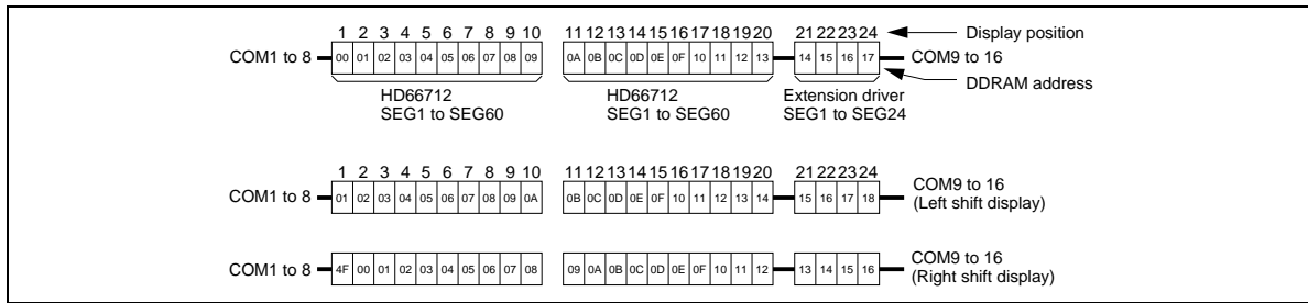
Figure 4 1-Line by 24-Character Display (6-Dot Font Width)
