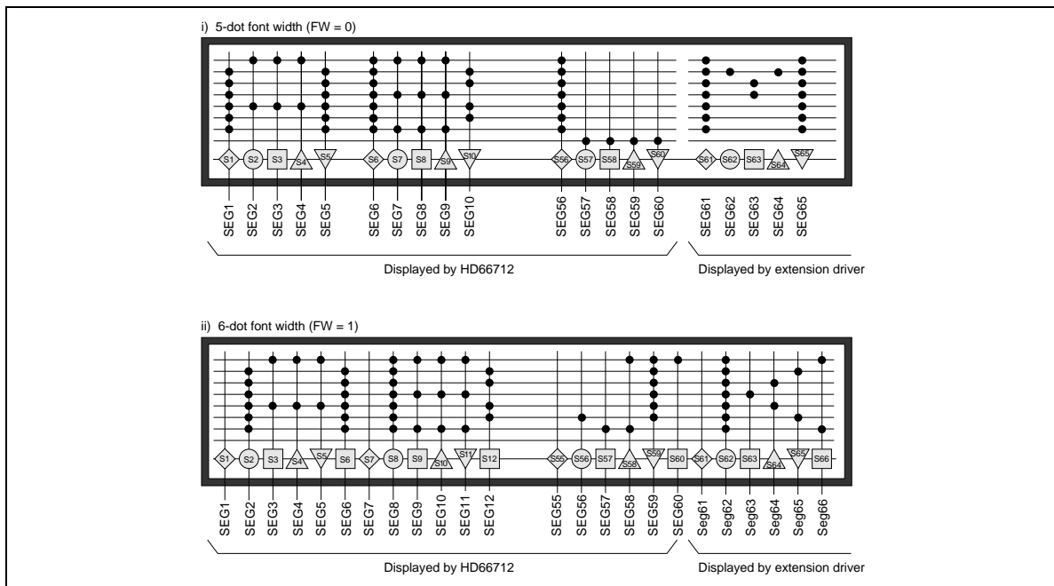
Figure 11 Correspondence between SEGGRAM and Segment Display
