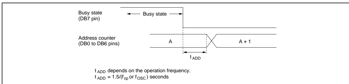
Figure 17 Address Counter Update
