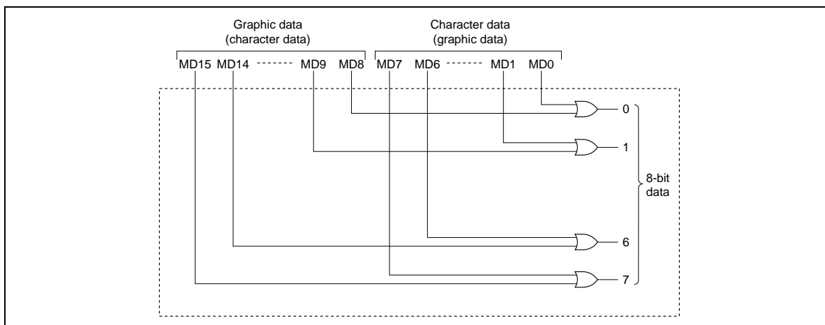
Figure 18 OR Function
