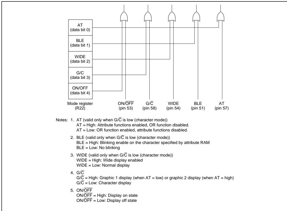
Figure 34 Correspondence between Mode Register and External Pins
