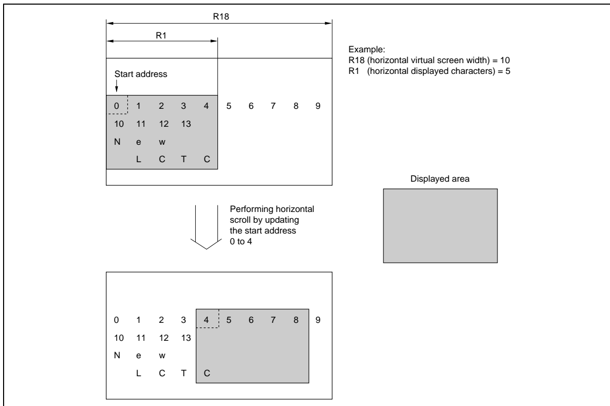
Figure 13 Example of Horizontal Scroll by Setting Horizontal Virtual Screen Width
