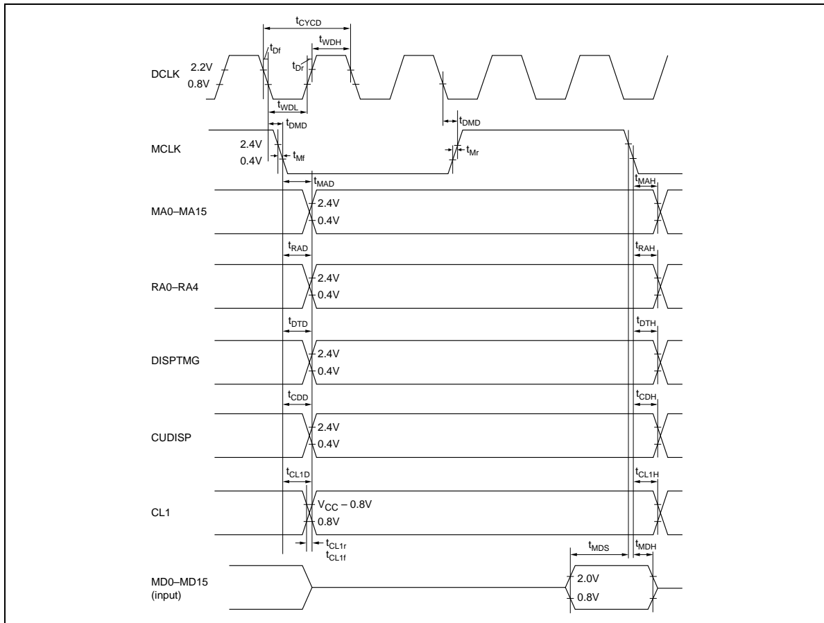
Figure 37 Memory Interface
