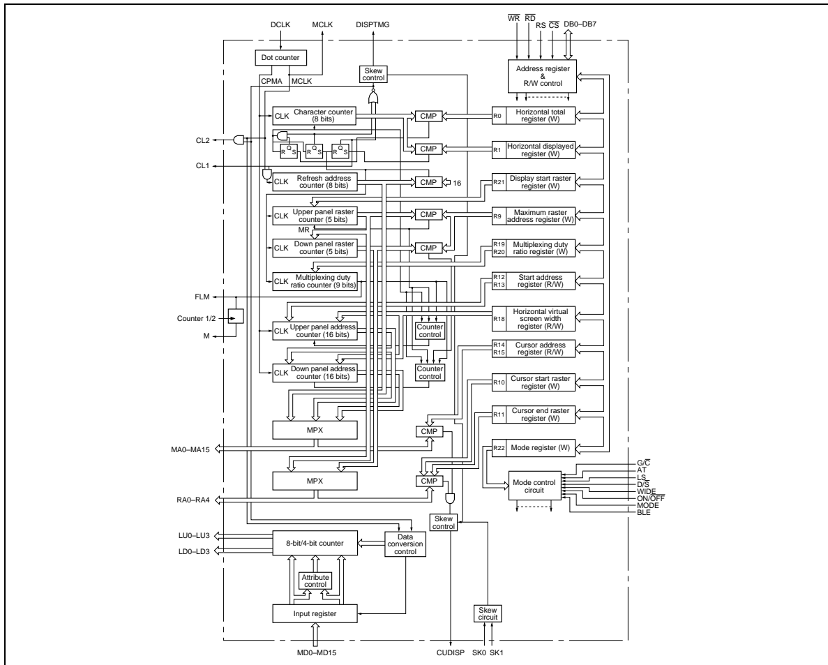
Figure 3 LCTC Block Diagram
