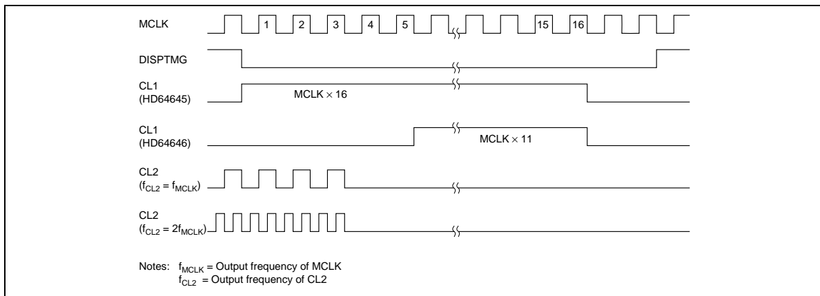
Figure 1 Differences between HD64645 and HD64646 (No Skew)
