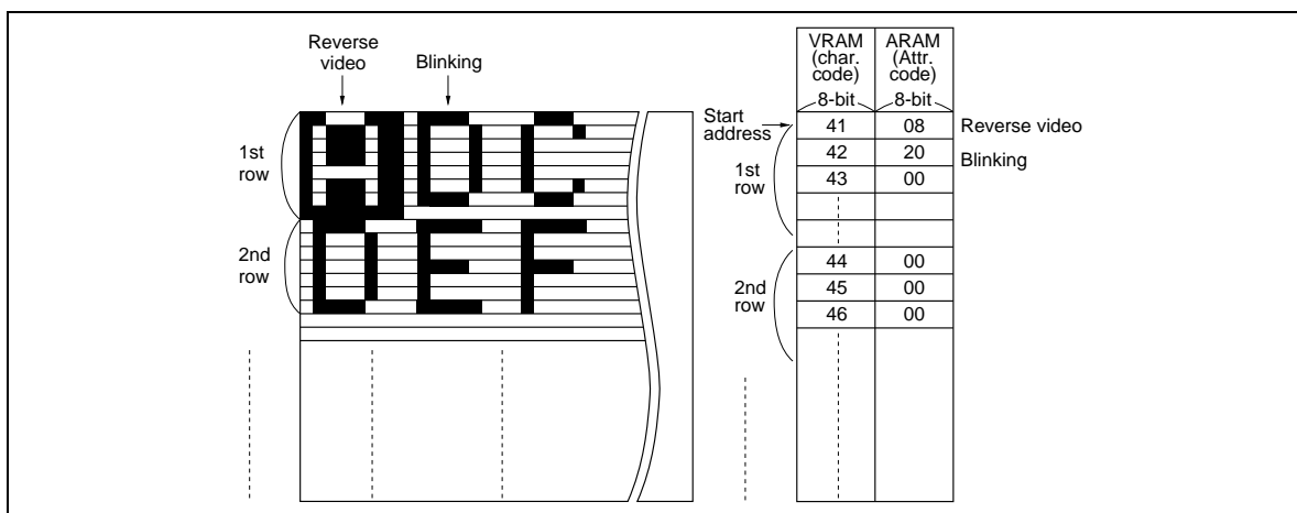
Figure 10 Relation between Character Screen and Memory Contents
