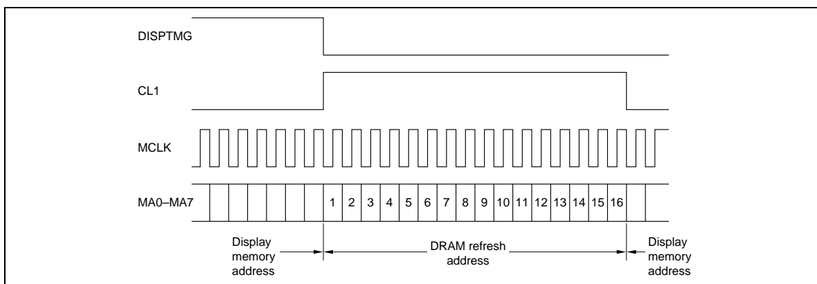
Figure 19 DRAM Refresh Address Output
