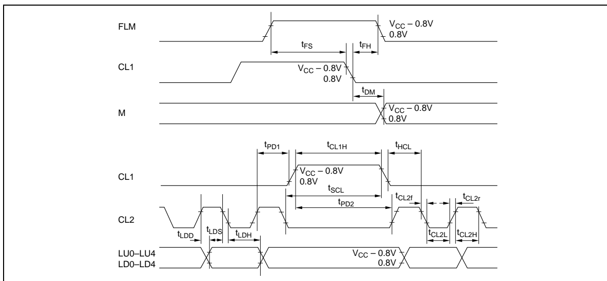
Figure 39 LCD Interface
