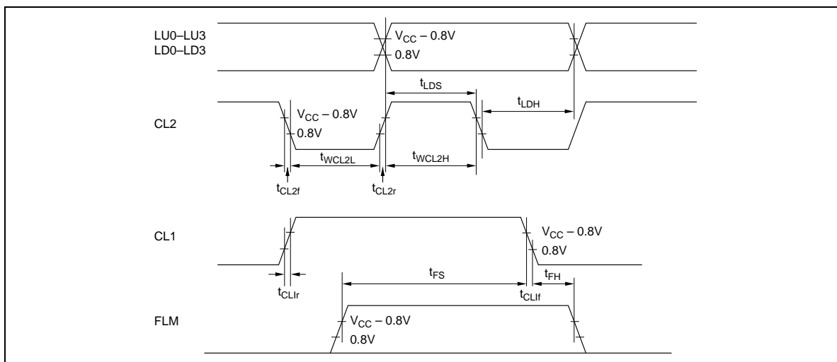
Figure 38 LCD Interface
