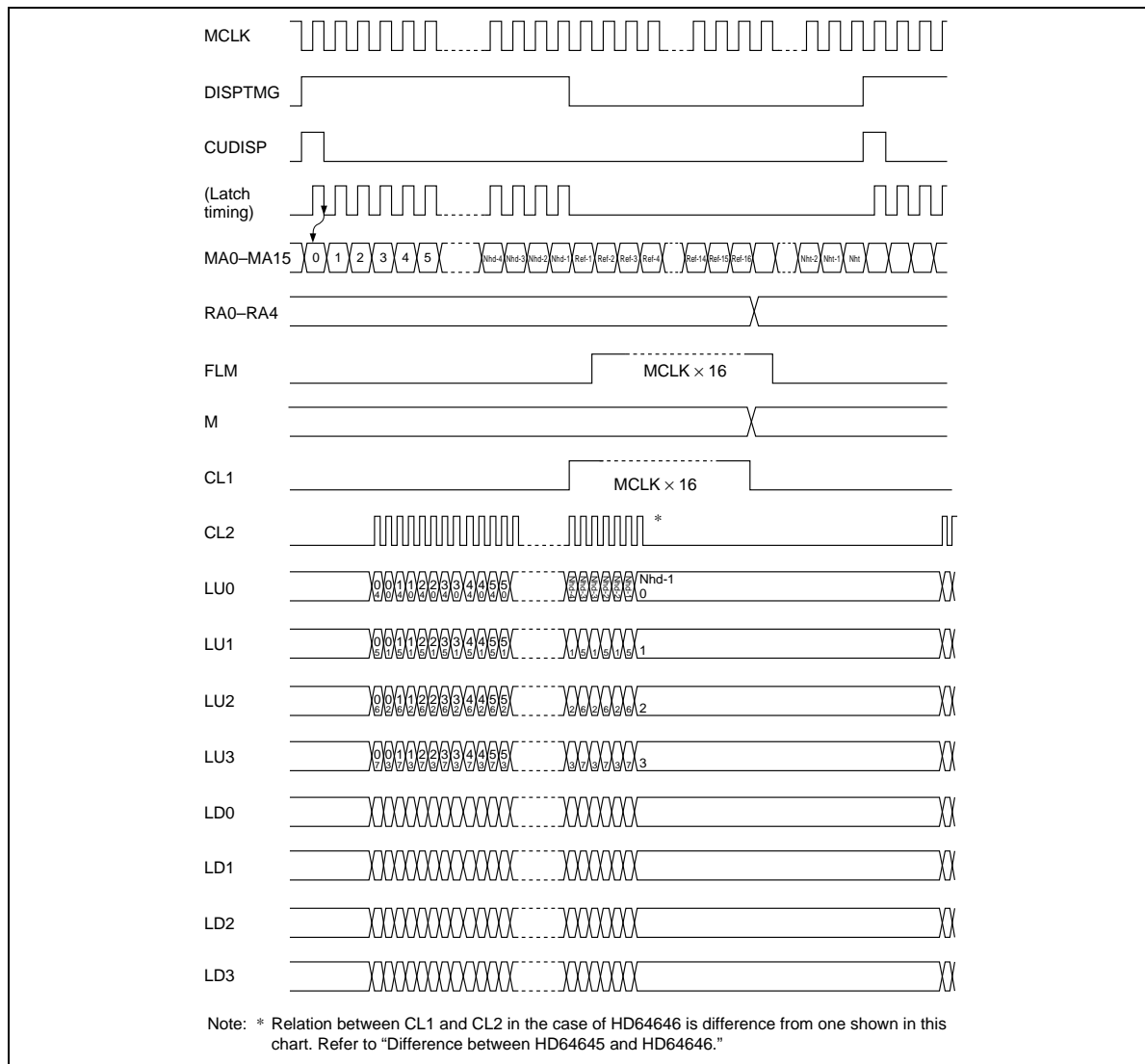
Figure 8 LCTC Timing Chart (In Mode 5: Single Screen, 4-Bit Transfer, Normal Character Display)
