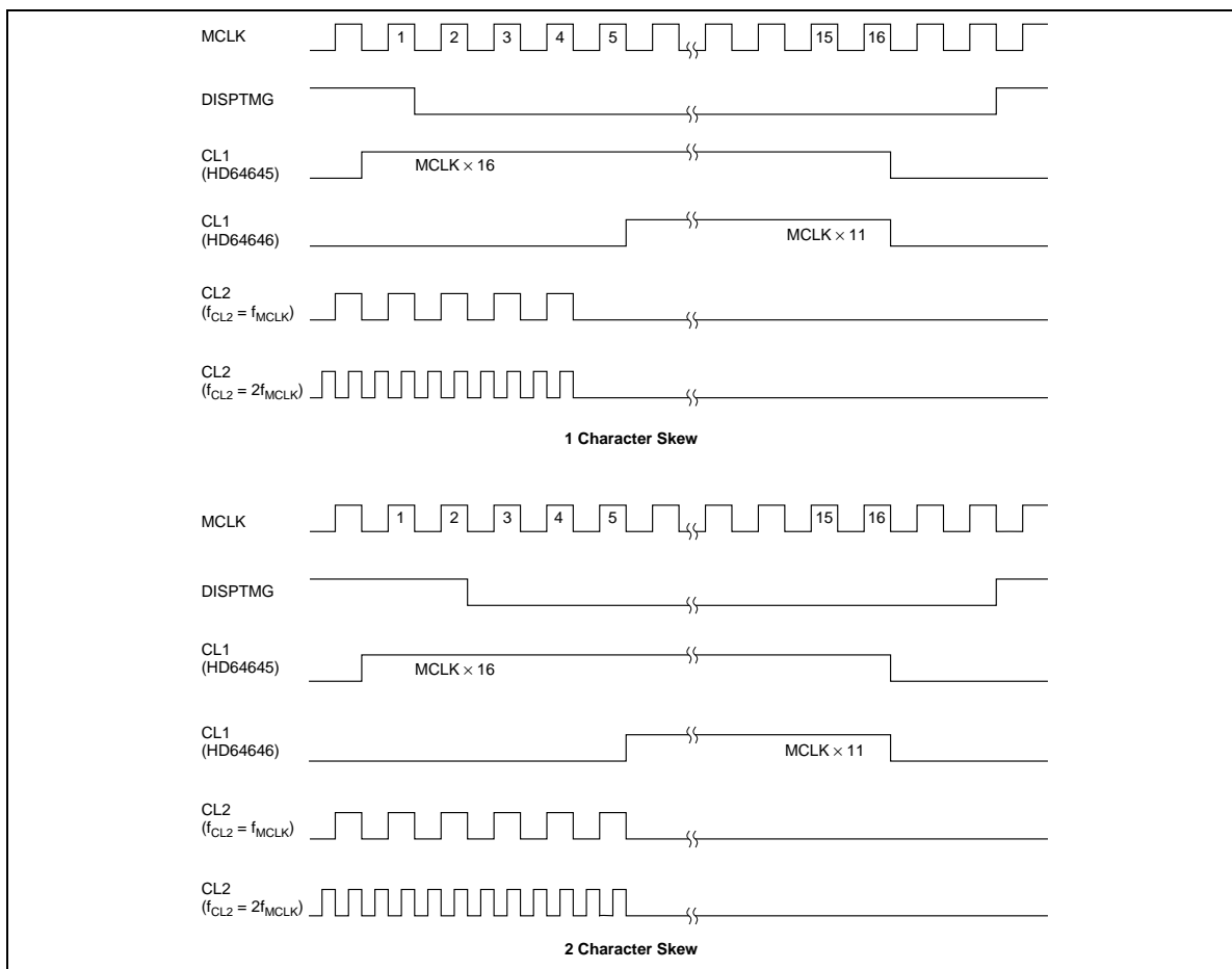
Figure 2 Differences between HD64645 and HD64646 (Skew)
