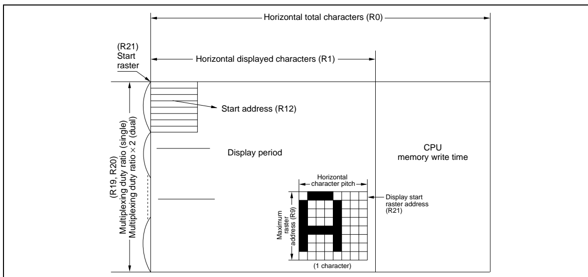
Figure 7 Relation between Display Screen and Registers
