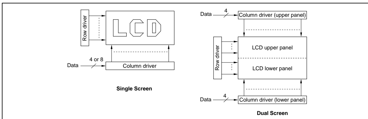
Figure 21 Hardware Configuration According to Screen Format
