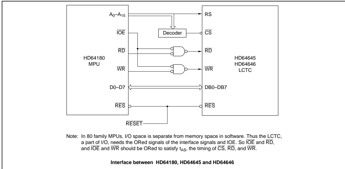
Figure 5 Interface to MPU
