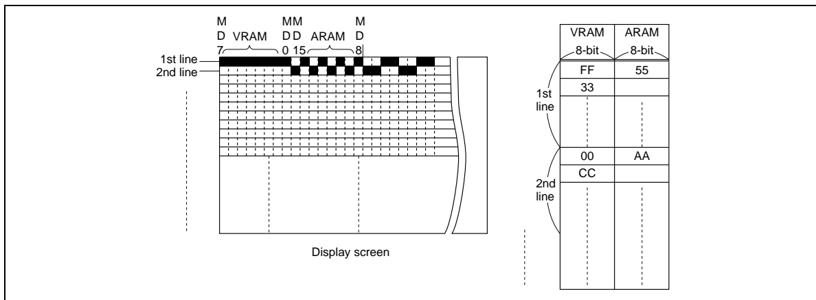
Figure 11 Relation between Graphic Screen and Memory Contents
