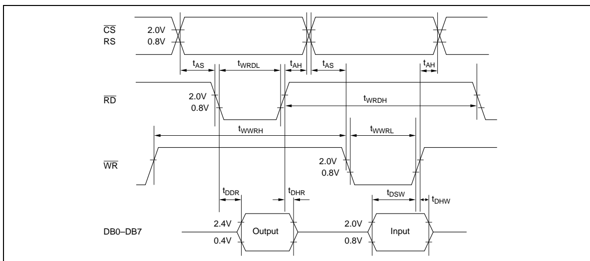
Figure 36 CPU Interface
