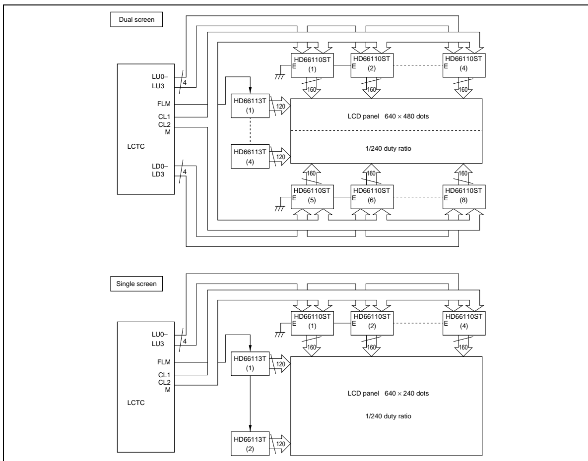
Figure 6 LCD Driver Examples
