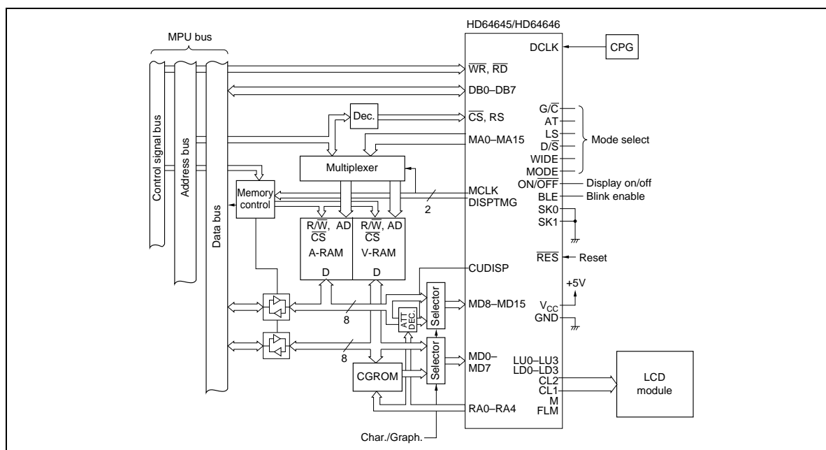
Figure 4 Character/Graphic Display System Example
