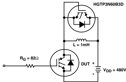
FIGURE 19. INDUCTIVE SWITCHING TEST CIRCUIT
