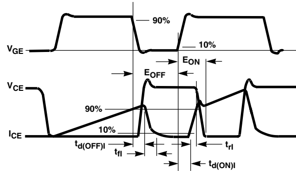
FIGURE 20. SWITCHING TEST WAVEFORMS
