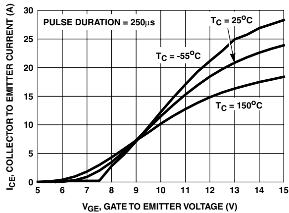
FIGURE 13. TRANSFER CHARACTERISTIC
