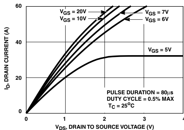
FIGURE 8. SATURATION CHARACTERISTICS
