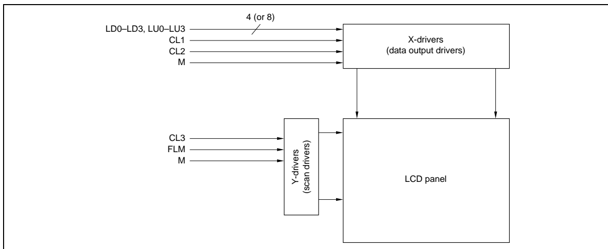
Figure 16 Connection for Double-Height Display
