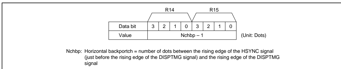
Figure 29 Horizontal Backporch Register
