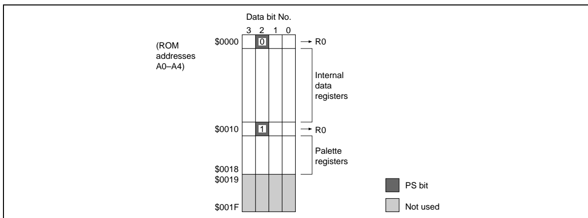
Figure 20 PS Bit Functions in ROM Programming Method
