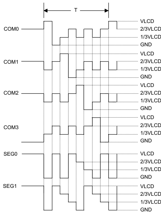
LCD timing
