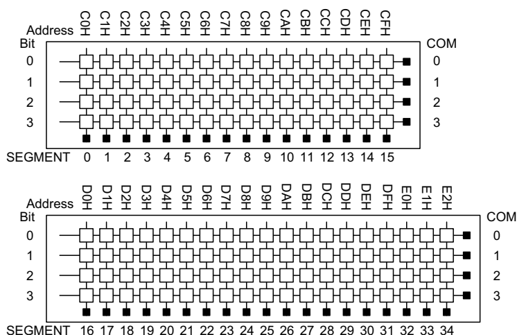
Display memory
