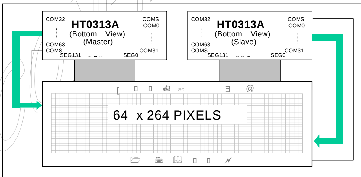
Figure 9-17. SHL = 1, ADC = 1
