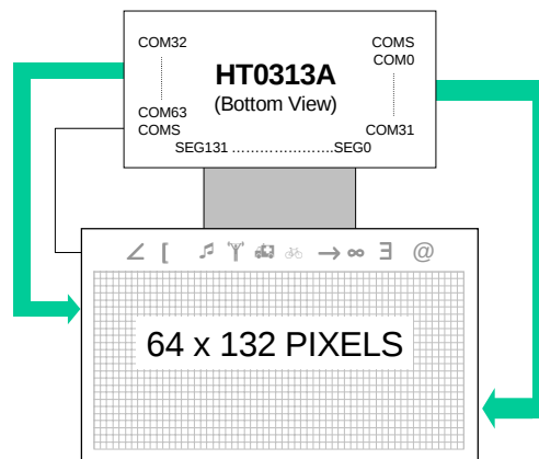
Figure 9-7. SHL = 1, ADC = 1
