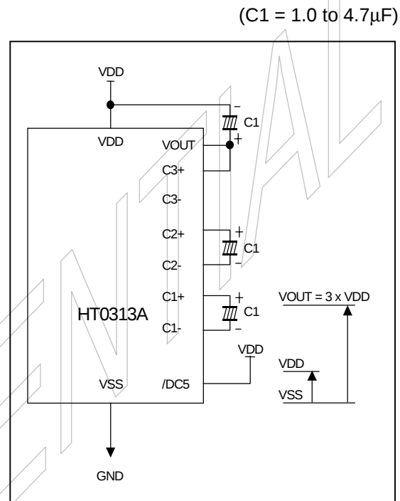
Figure 6-10. Three times boosting circuit
