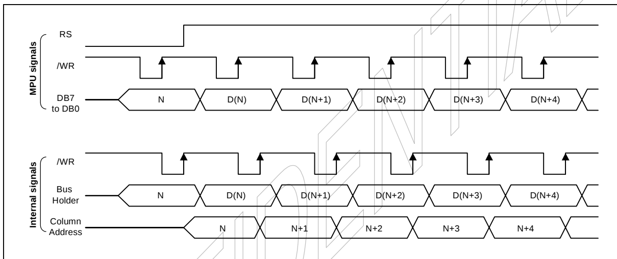
Figure 6-2. Write timing
