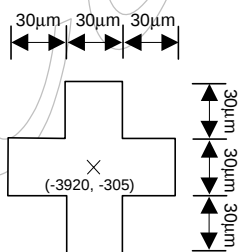
Figure 4-2. COG align key
