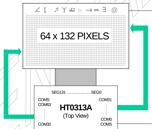
Figure 9-5. SHL = 0, ADC = 1
