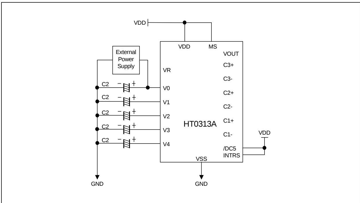
Figure 6-17. When using some LCD power circuits (V/C: OFF, V/R: OFF, V/F: ON)
