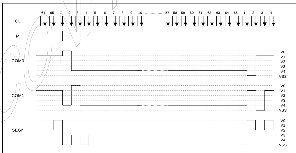
Figure 6-7. 2-frame AC driving waveform (Duty ratio = 1/65)
