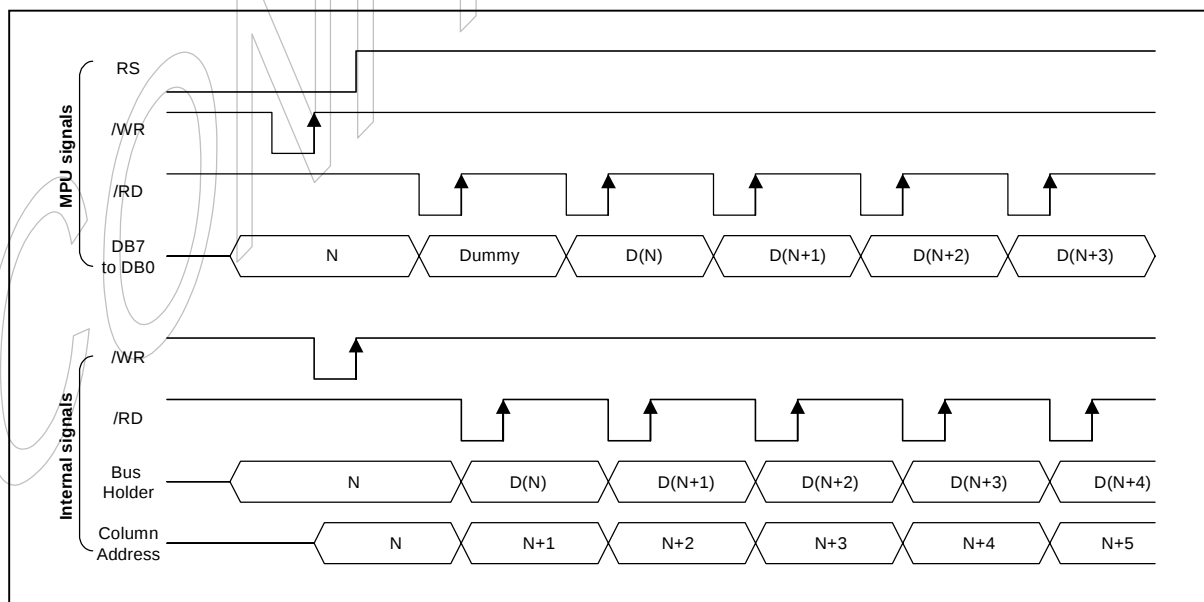
Figure 6-3. Read timing
