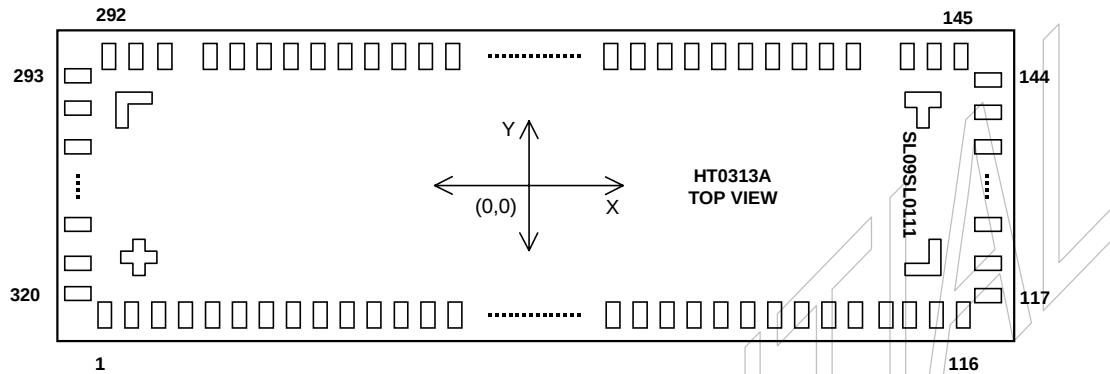
Figure 4-1. Chip configuration
