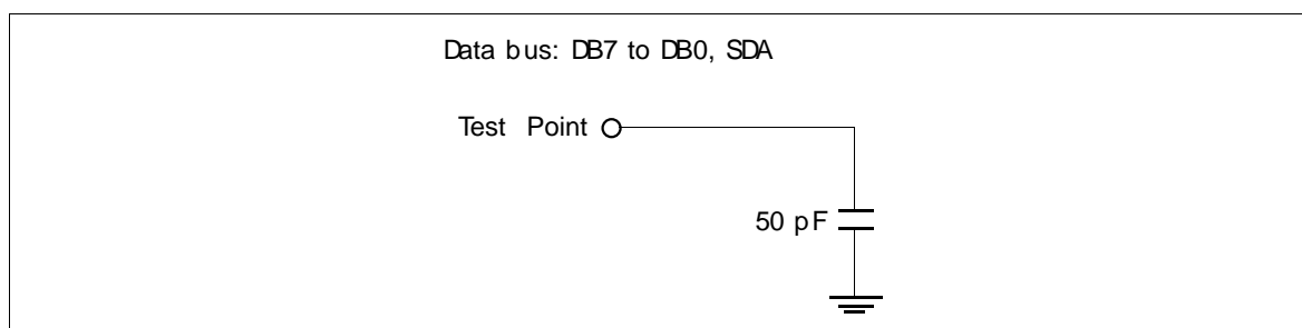
Figure 47 Load Circuit
