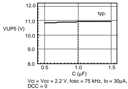
Figure 46 Booster (cont)
