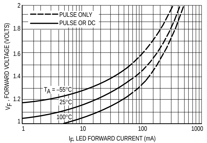
Figure 4. LED Forward Characteristics
