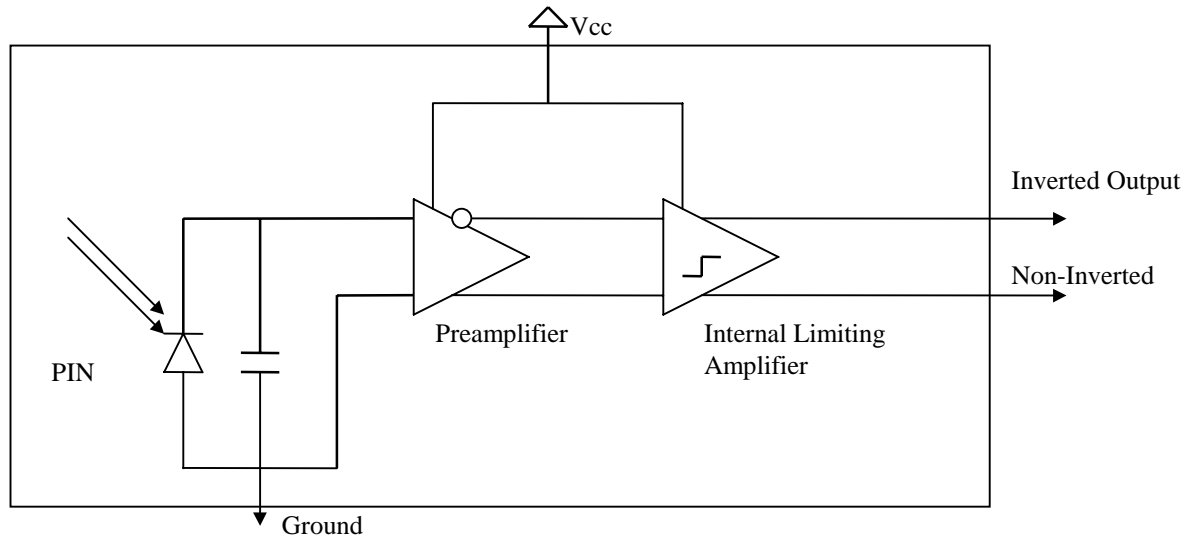
FIGURE 1: INTERNAL SCHEMATIC DIAGRAM OF THE HFD3180-002
