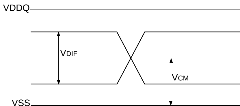
Figure 1. Diffrential Voltage / Common Mode Voltage
