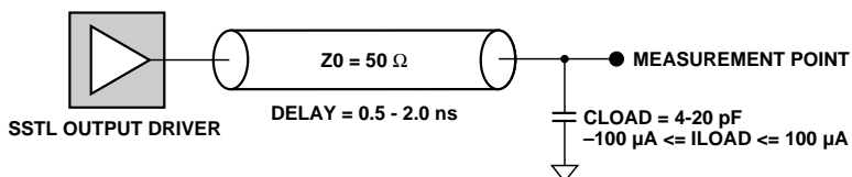
Figure 5. Test conditions for SSTL_2 and SSTL_3 output drivers.
