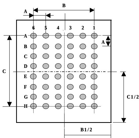
BUMP VIEW
