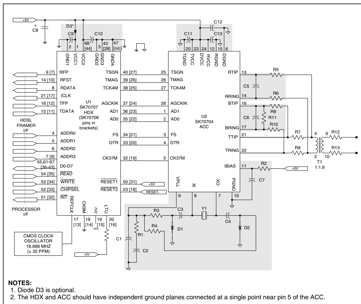
Figure 14. Typical Support Circuitry for LTU Applications
