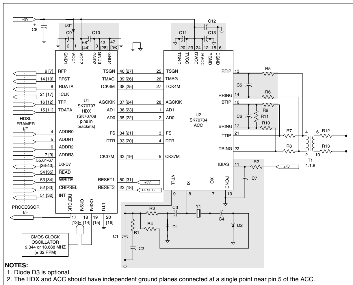
Figure 15. Typical Support Circuitry for NTU Applications
