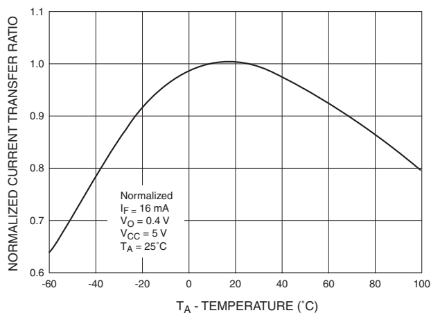
Fig. 4 Current Transfer Ratio vs. Temperature
