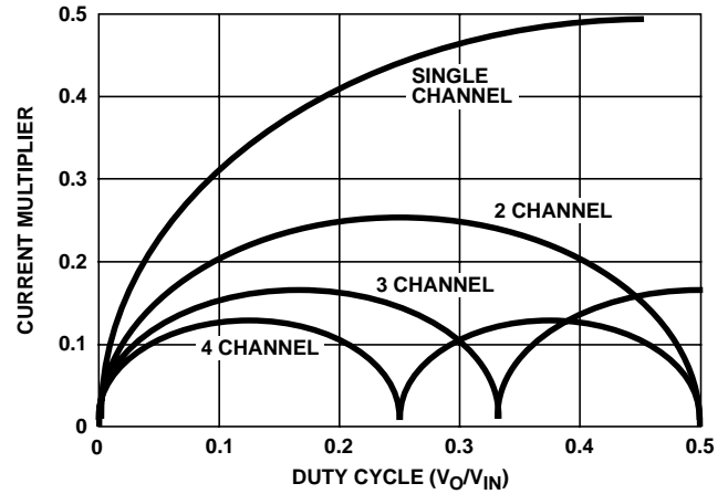
FIGURE 13. CURRENT MULTIPLIER vs DUTY CYCLE
