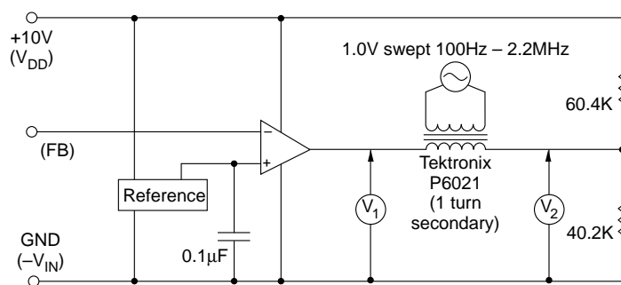
Error Amp Z_{OUT}
