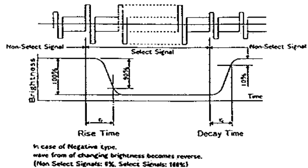
Ⓒ Definition of Optical Response Time
