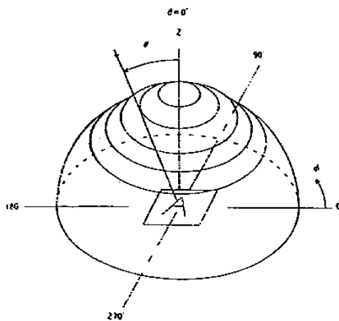
Ⓐ Definition of Viewing Angle θ and φ
