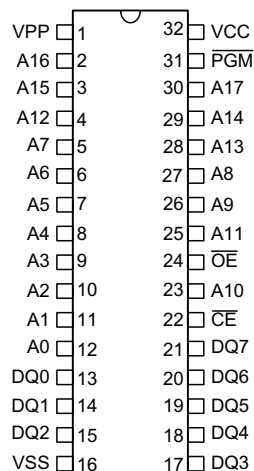
HT27C020 - 32 DIP/SOP
