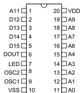
HT6207 – 20 DIP/SOP
