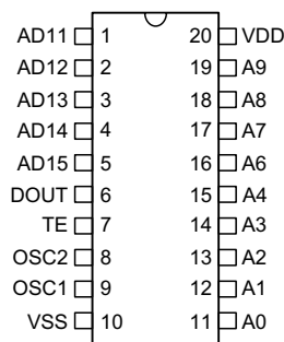
HT600 – 20 DIP/SOP
