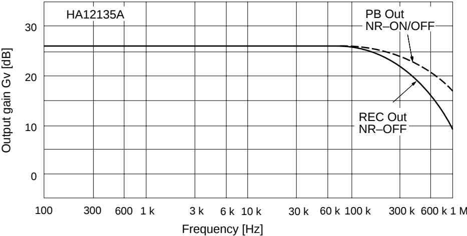
Figure 16 REC Mode Output Gain vs. Frequency
