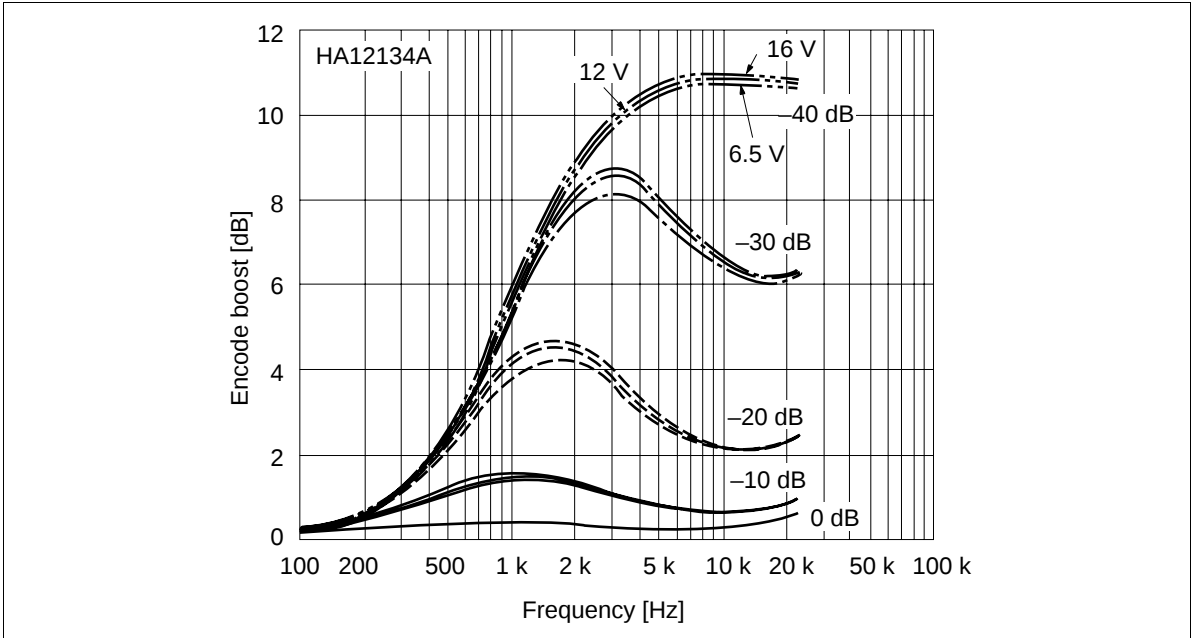
Figure 26 Encode Boost vs. Frequency
