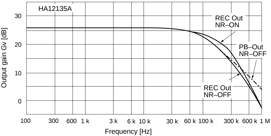
Figure 17 PB Mode Output Gain vs. Frequency
