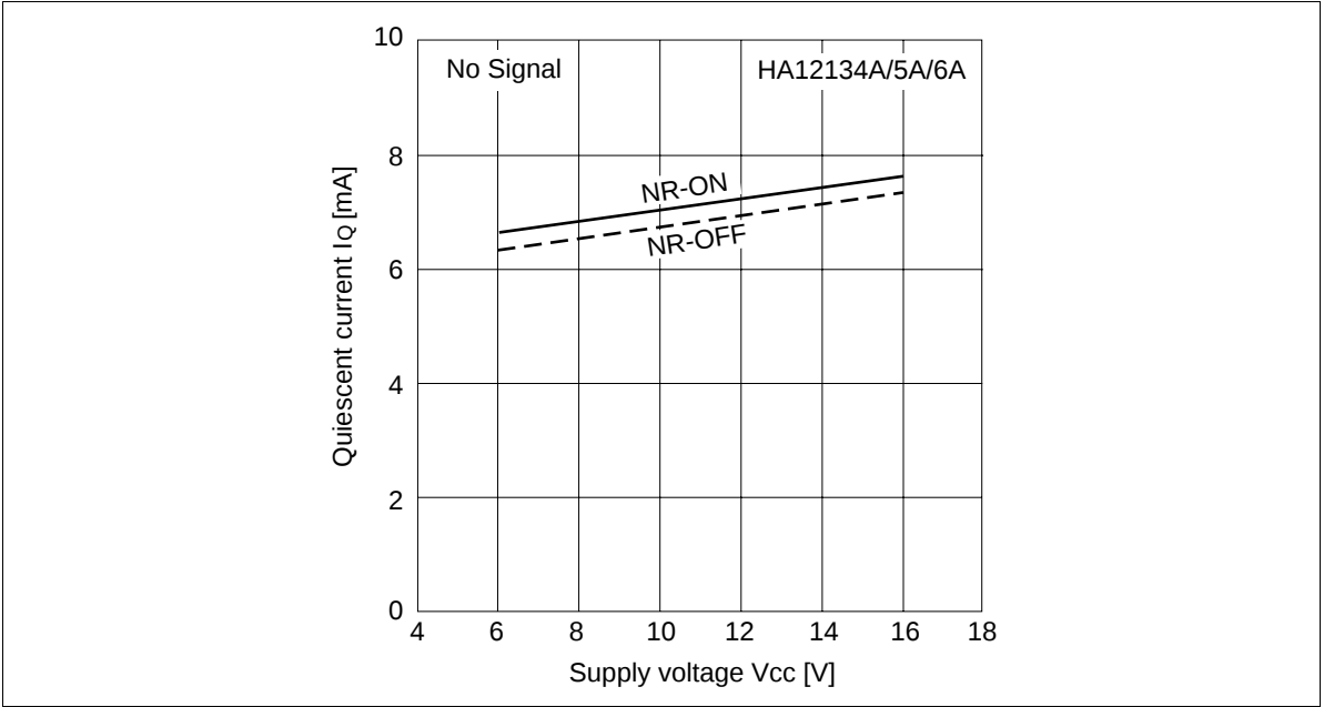
Figure 1 Quiescent Current vs. Supply Voltage
