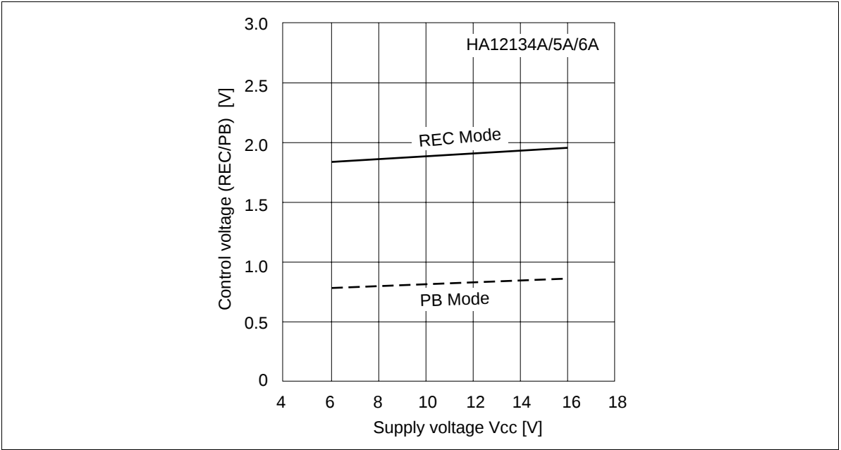
Figure 2 REC/PB Control Voltage vs. Supply Voltage
