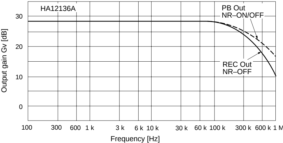
Figure 5 REC Mode Output Gain vs. Frequency
