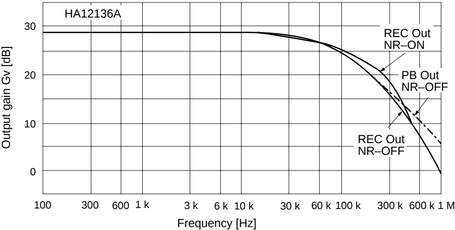
Figure 6 PB Mode Output Gain vs. Frequency
