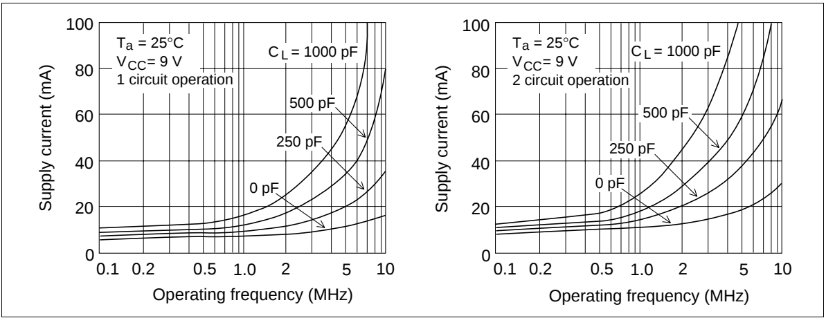
Supply current vs. operating frequency (HD29028)
