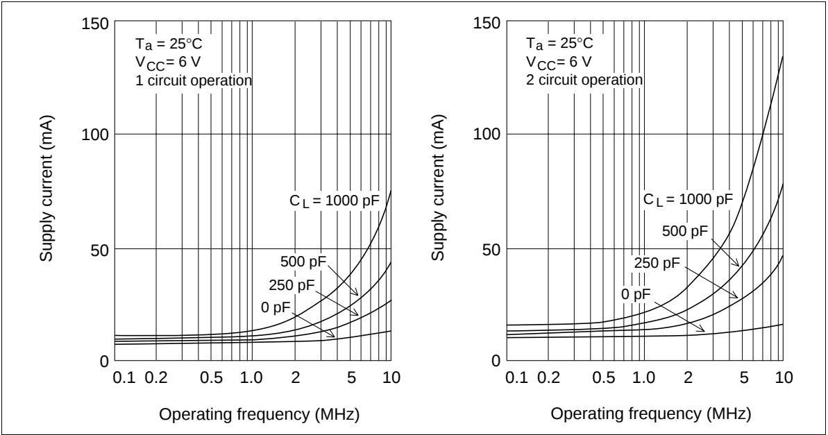
Supply current vs. operating frequency (HD29028)
