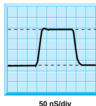
PULSE RESPONSE (0dBm INPUT)
