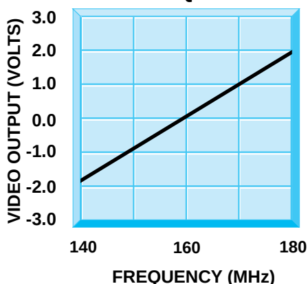
VIDEO OUTPUT vs. FREQUENCY
