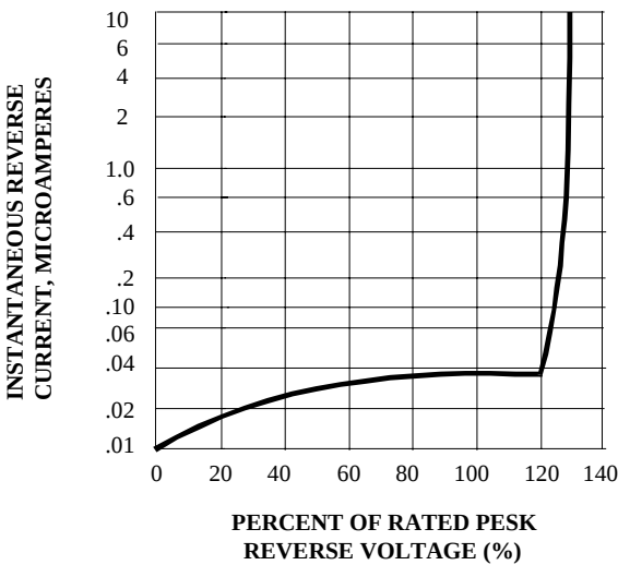
FIG. 2 - TYPICAL REVERSE CHARACTERISTICS 25°C T A
