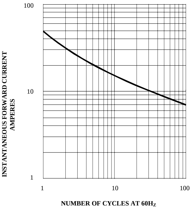
FIG. 3 - PEAK FORWARD SURGE RATING
