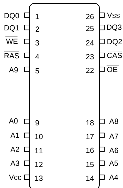
20/26 Pin Plastic TSOP- II (300mil)
