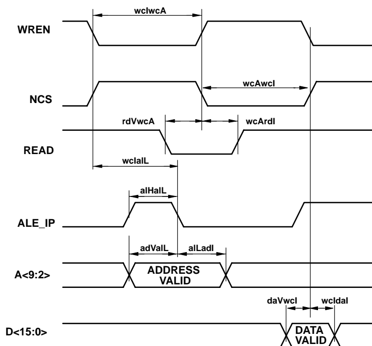
Fig. 38 : Motorola mode write, ALE_IP non-overlapping WREN and NCS (NARMSYS = 1, NINTELMOT = 1, WRPROG = X)
