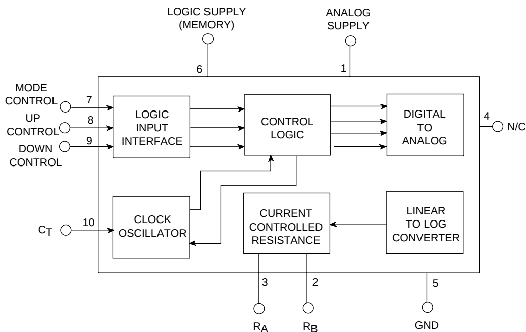
BLOCK DIAGRAM
