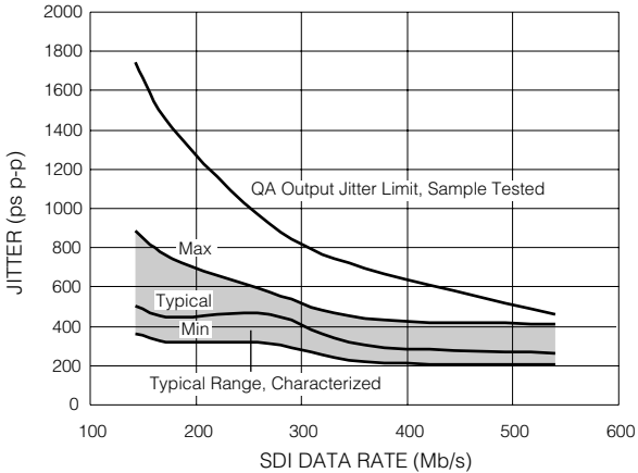
Fig. 7 Intrinsic Jitter - Pathological SDI Checkfield
