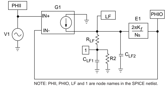
Fig. 18 SPICE Model of PLL
