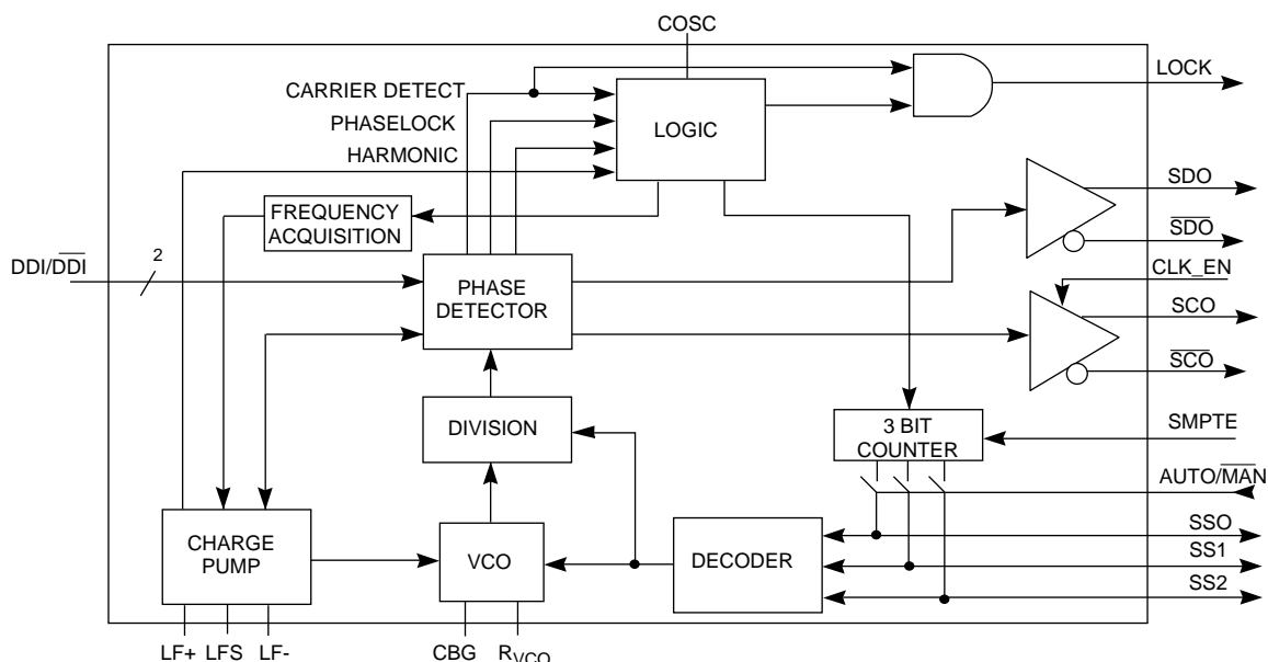
BLOCK DIAGRAM
