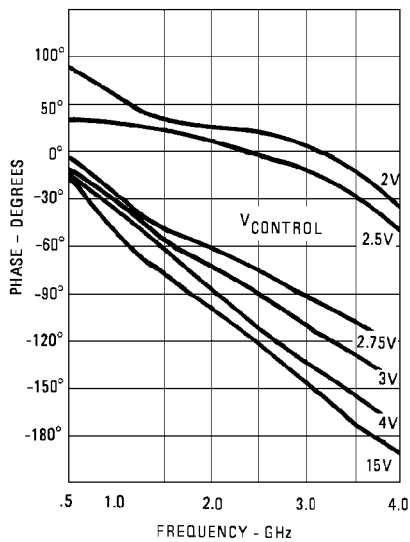
Phase vs. V_{\text{CONTROL}} vs. Frequency
