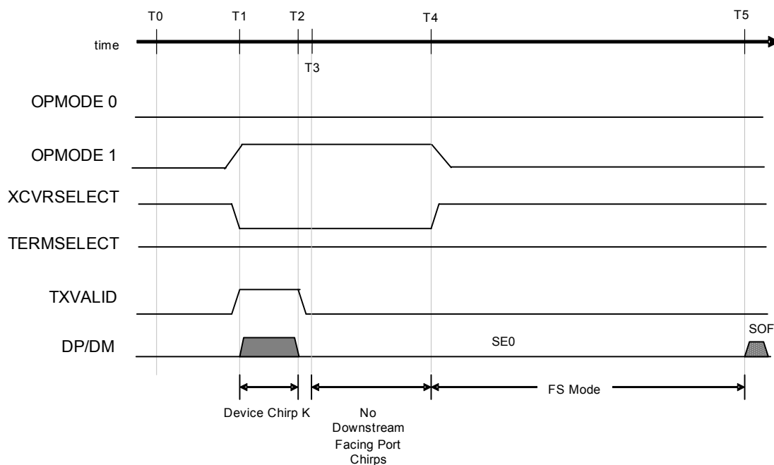
Figure 8.3 - HS Detection Handshake Timing Behavior (FS Mode)
