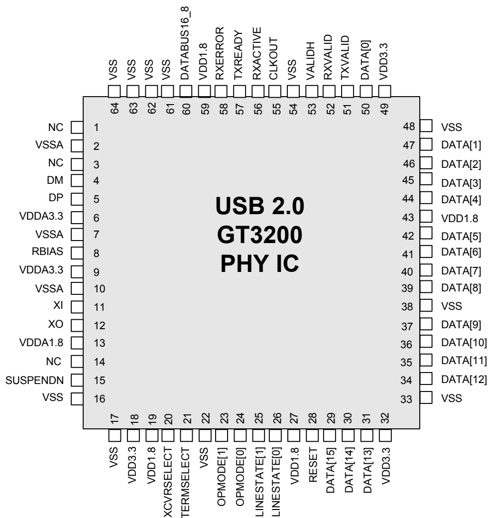
Figure 3.1 - GT3200 Pinout
