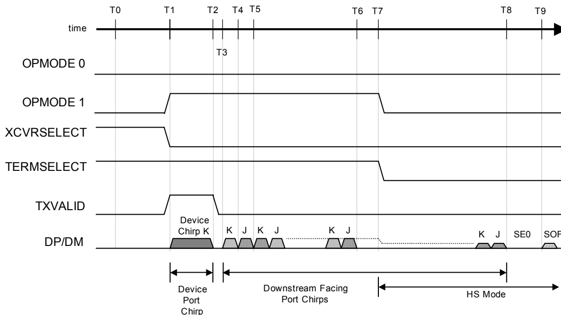
Figure 8.5 - HS Detection Handshake Timing Behavior (HS Mode)
