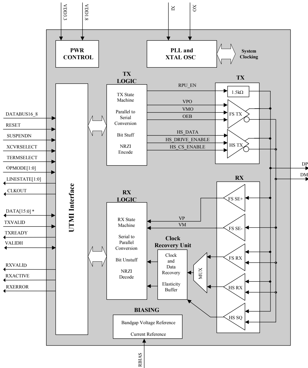
Figure 2.1- Block Diagram
