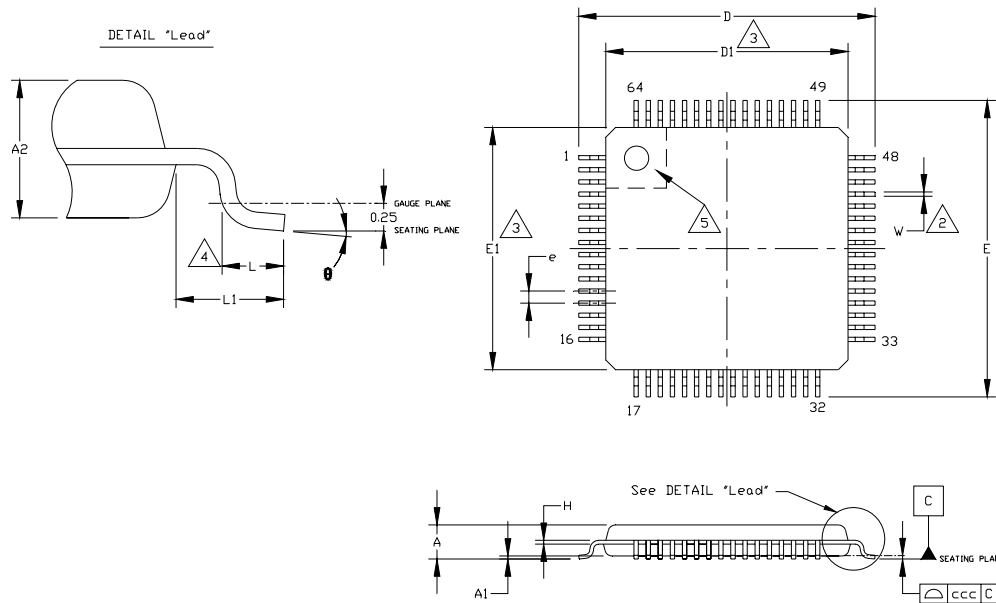
Figure 9.2 - GT3200-JN 64 Pin TQFP Package Outline, 7x7x1.4mm Body
