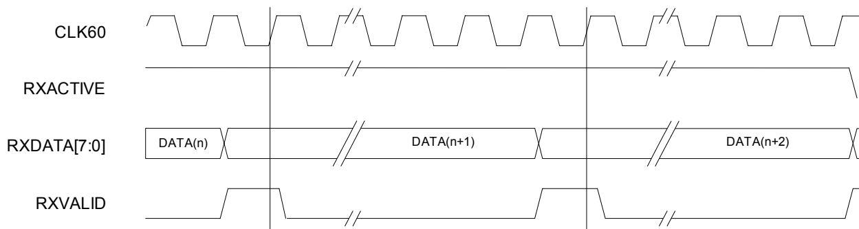
Figure 7.3 - FS CLK Relationship to Receive Data and Control Signals (8-bit mode)
