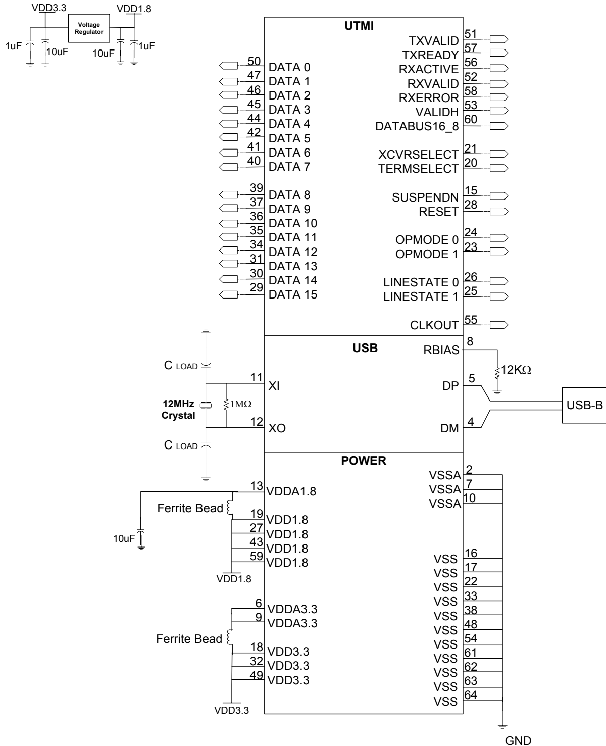
Figure 8.9 - Application Diagram
