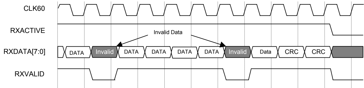
Figure 7.7 - Receive Timing for Data with Unstuffed Bits (8-bit mode)
