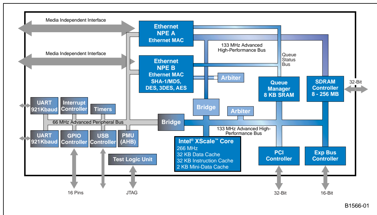
Figure 3. Intel® IXP421 Network Processor: Block Diagram
