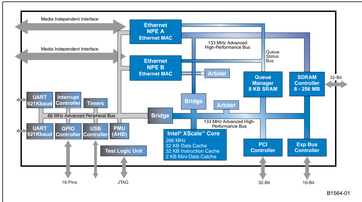
Figure 4. Intel® IXP420 Network Processor and IXC1100 Control Plane Processor: Block Diagram
