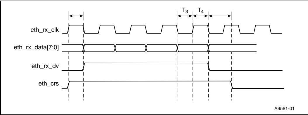
Figure 20. MII/RMII Input Timings
