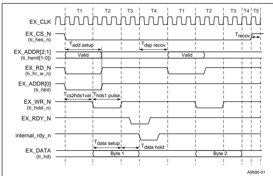
Figure 29. HPI – 8 Mode Write Accesses
