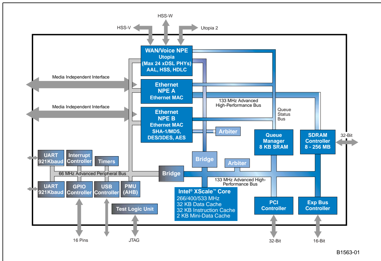
Figure 1. Intel® IXP425 Network Processor: Block Diagram
