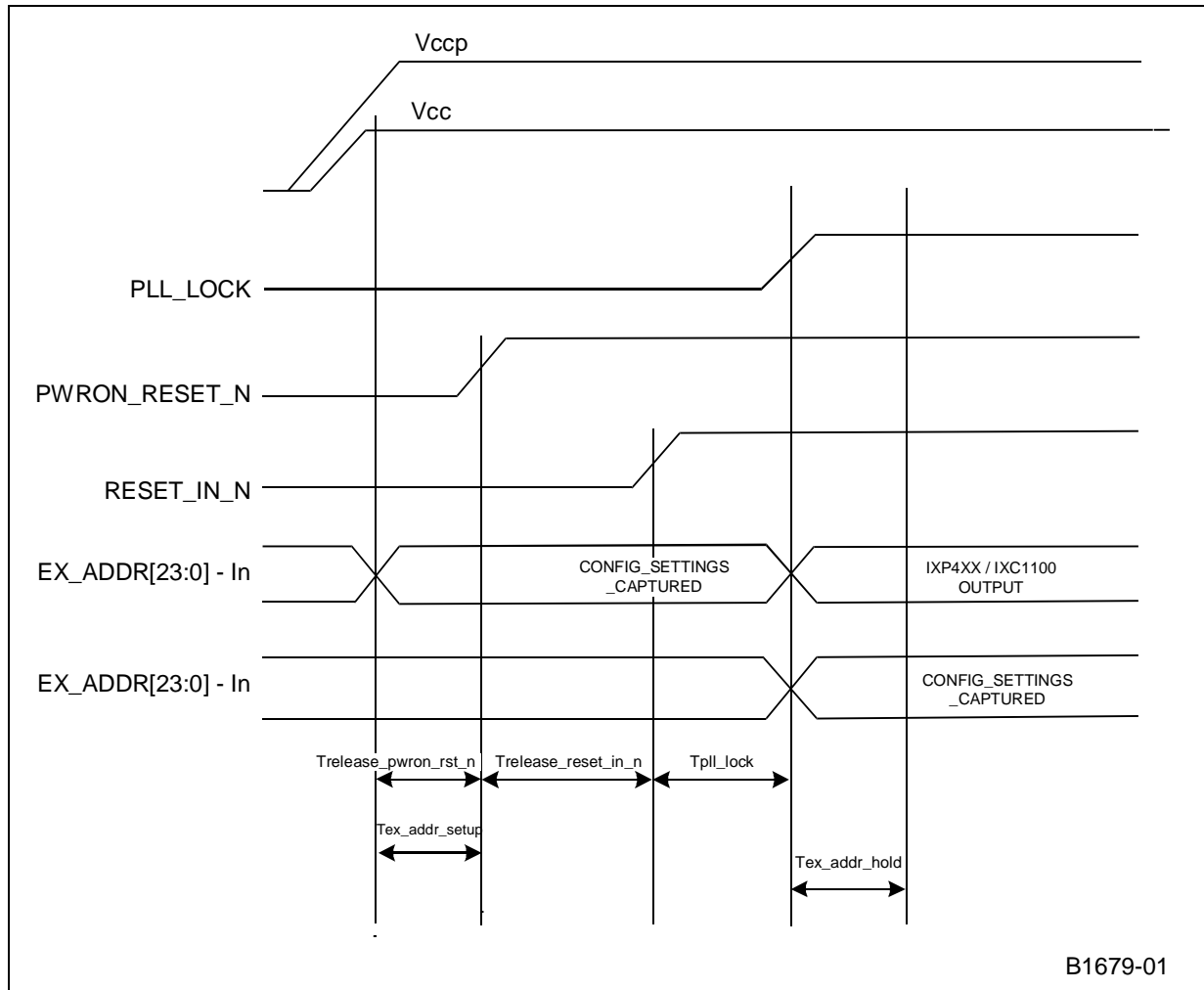
Figure 37. Reset Timings
