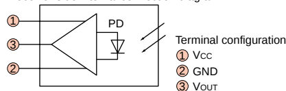
Receiver-side internal connection diagram
