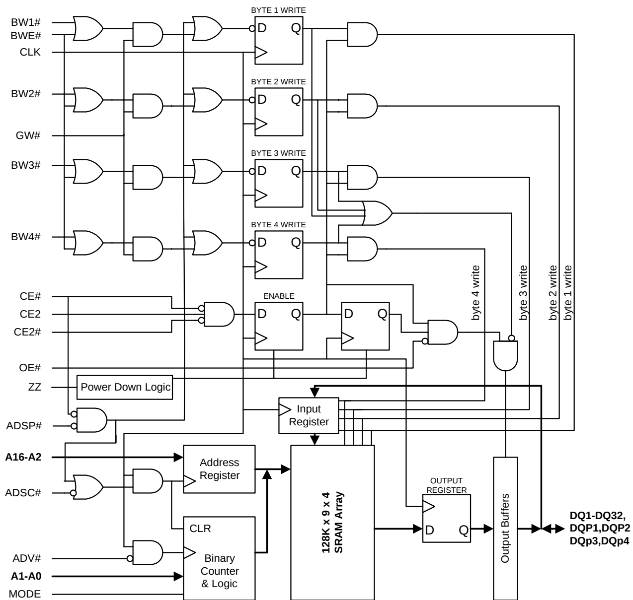
128K x 36 (CY7C1347A/GVT71128G36) Functional Block Diagram [1]
