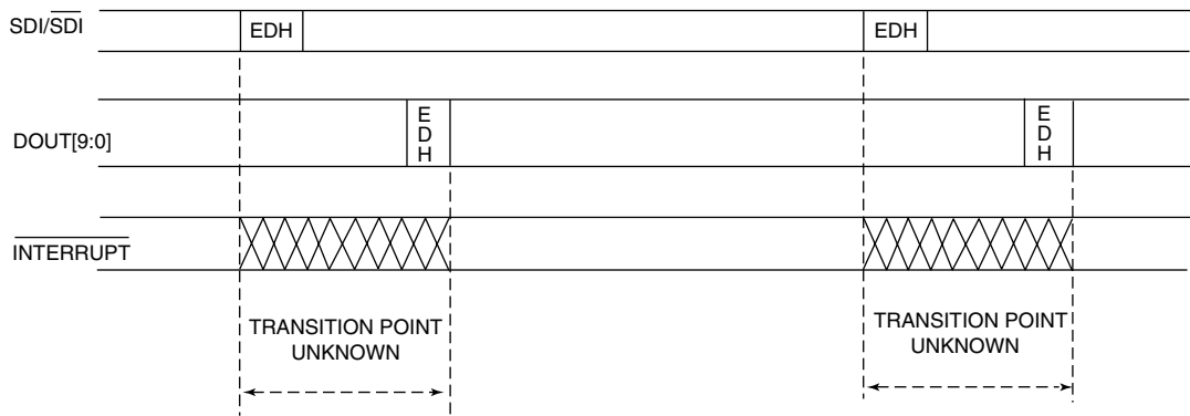
Fig. 11 \overline{\text{INTERRUPT}} Timing
