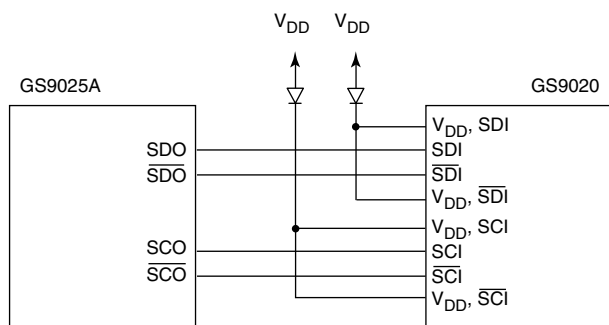
Fig. 5 Interfacing the GS9020 to the GS9025A
