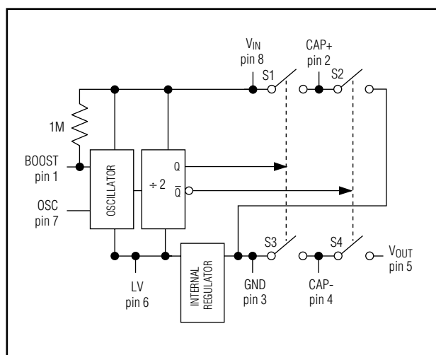
Fig. 10 – Functional Diagram
