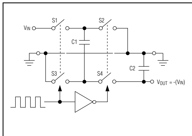
Fig. 7 – Ideal Voltage Inverter
