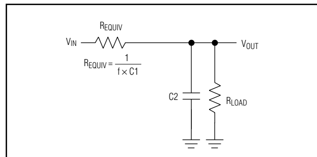
Fig. 9 – Equivalent Impedance
