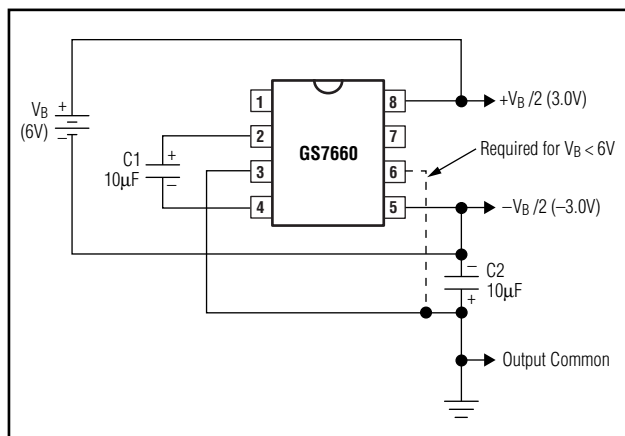
Fig. 13 – Battery Splitter
