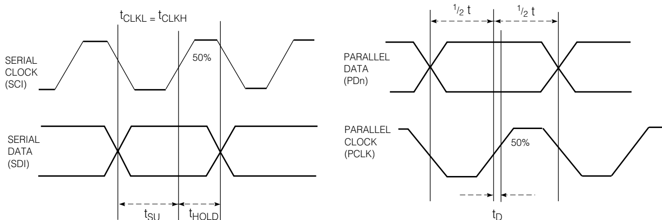
Fig. 7 Waveforms
