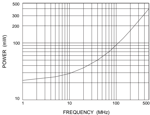
Fig. 8 Power Consumption
