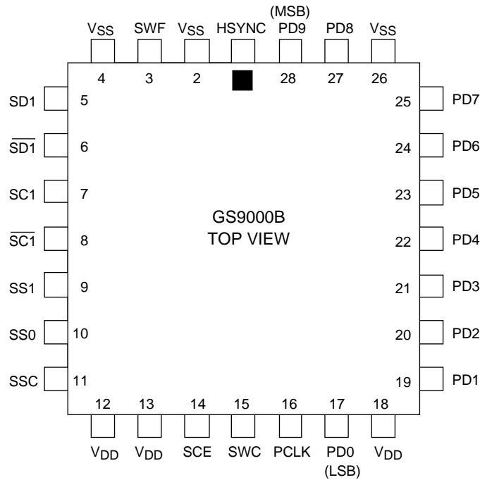
Fig. 1 GS9000B Pin Outs, 28 Pin PLCC Package
