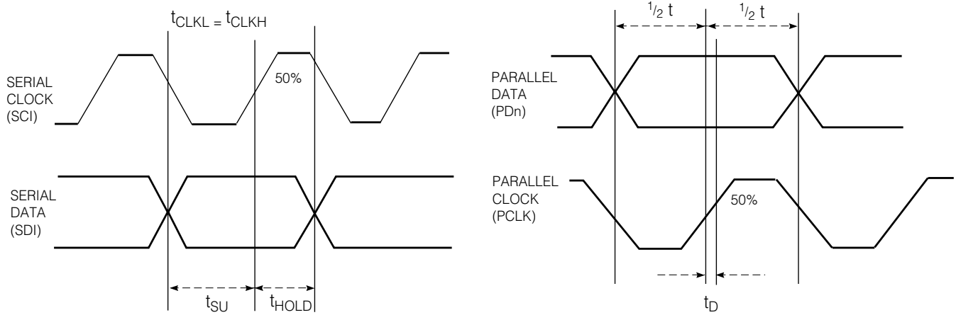
Fig. 7 Waveforms
