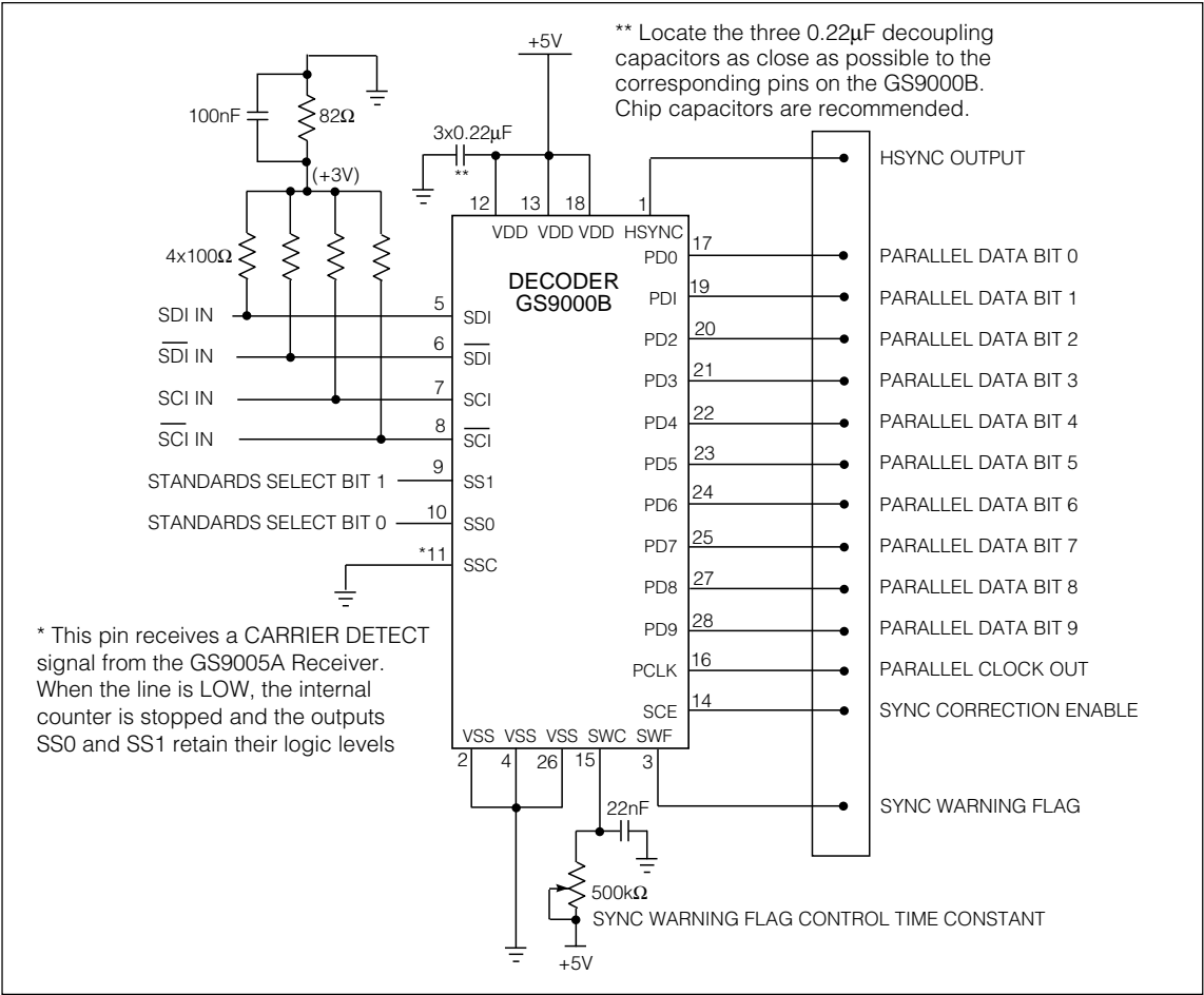
Fig. 9 GS9000B Test Set-Up
