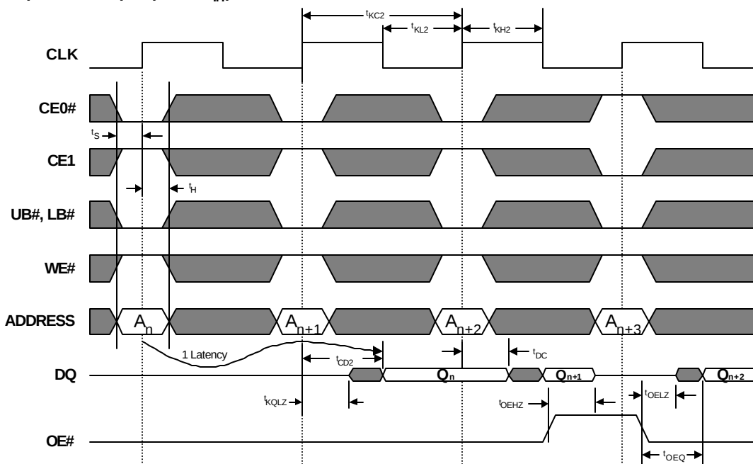
Read Cycle for Pipelined Output (FT# = V_{IH} ) [1, 2, 3, 4, 5]
