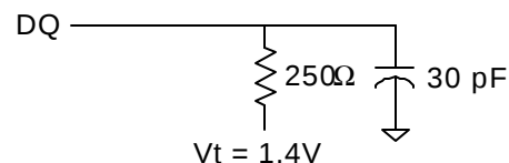
Fig. 1 OUTPUT LOAD EQUIVALENT
