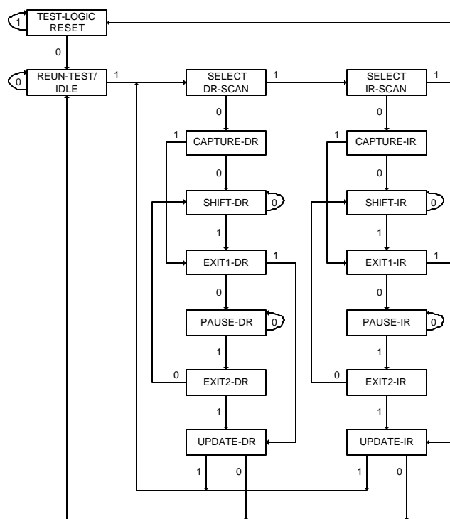
Figure 3 TAP CONTROLLER STATE DIAGRAM
