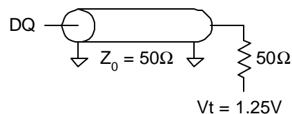
Fig. 1A OUTPUT LOAD EQUIVALENT
