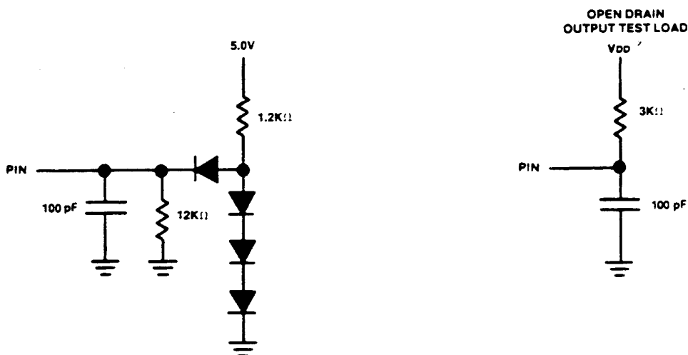
Figure 13. Test Load
