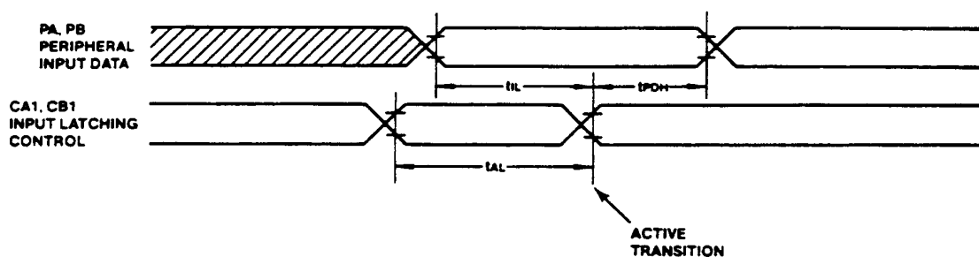
Figure 8. Peripheral Data, Input Latching Timing
