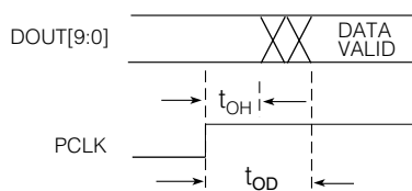
Fig. 15: Video Data Output Delay &amp; Hold Times
