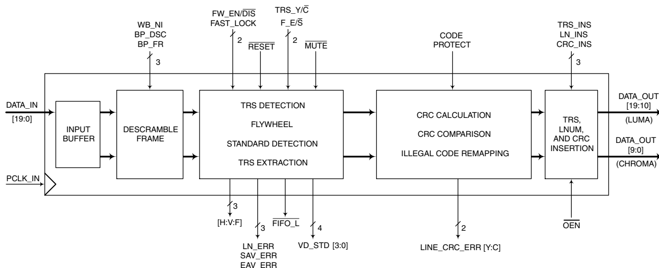
BLOCK DIAGRAM
