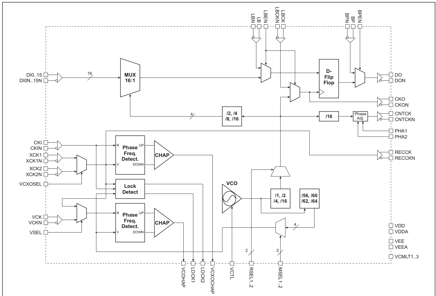
Figure 14. GD16557 - Block diagram
