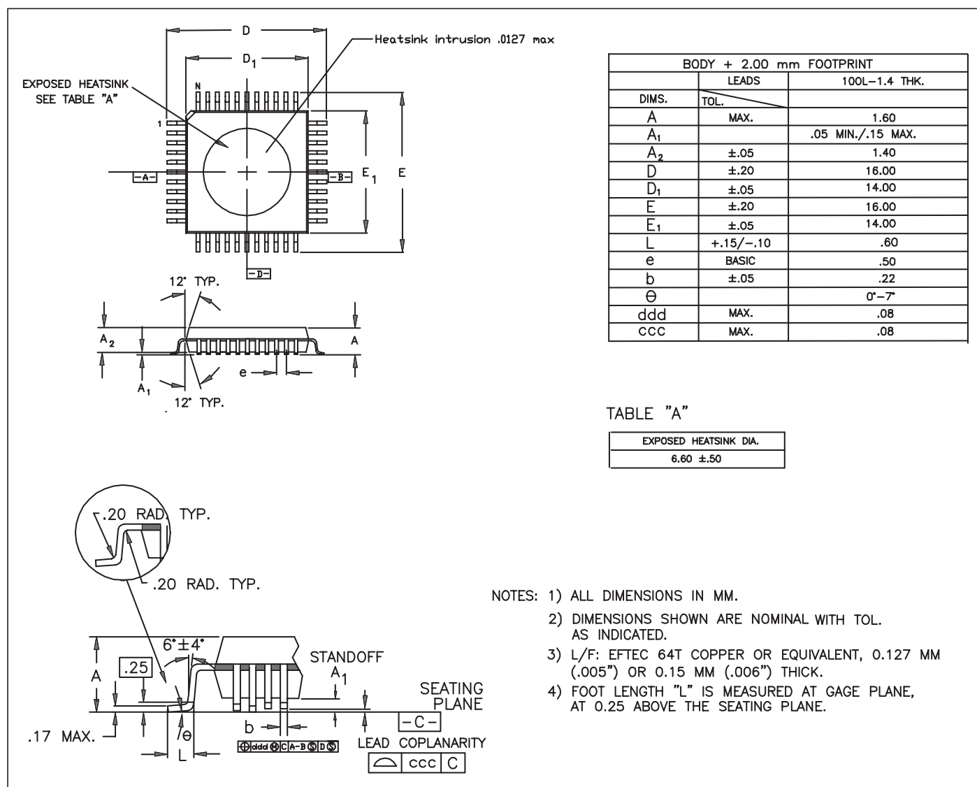
Figure 32. 100 pin TQFP-EDQUAD. All dimensions are in mm.
