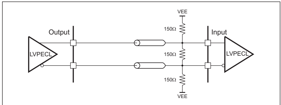
Figure 7. LVPECL output termination, DC-coupled.
