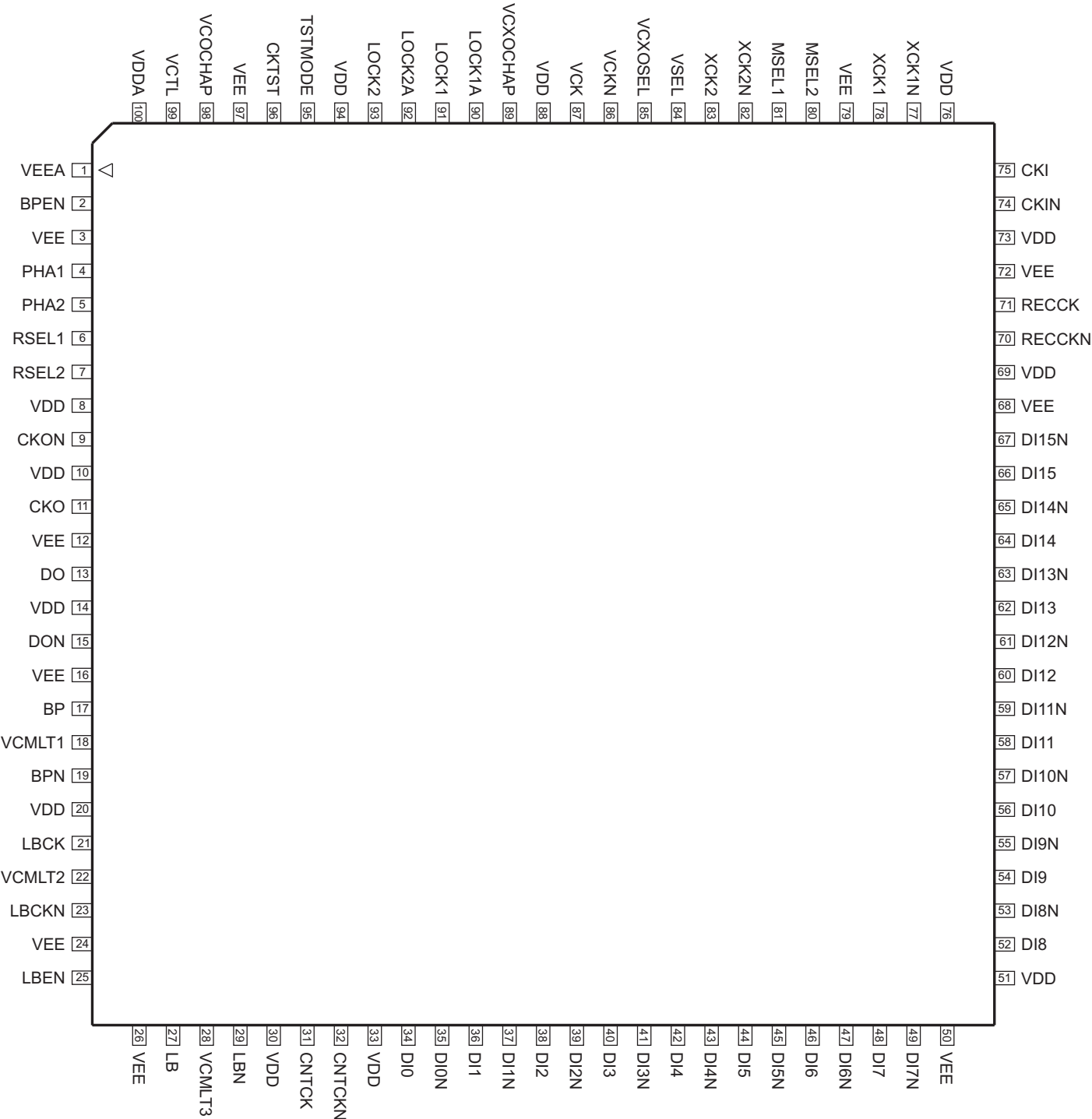
Figure 24. Package Pinout, 100 pin. Top view.
