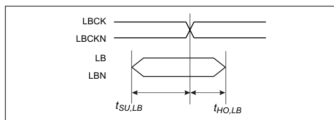
Figure 30. Loop-back timing.
