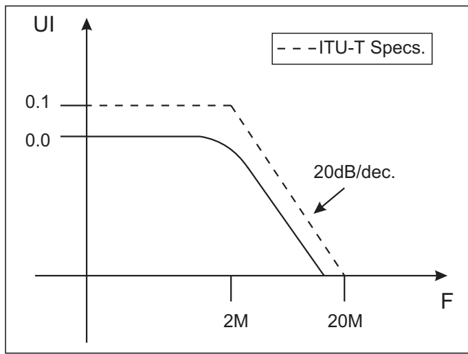
Figure 27. Jitter Transfer
