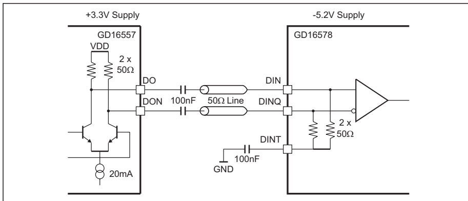
Figure 17. GD16557/GD16578 AC-connection
