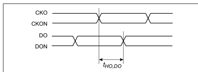
Figure 31. High-speed clock/data timing
