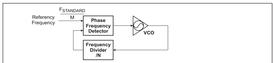
Figure 3. Basic PLL frequency synthesis
