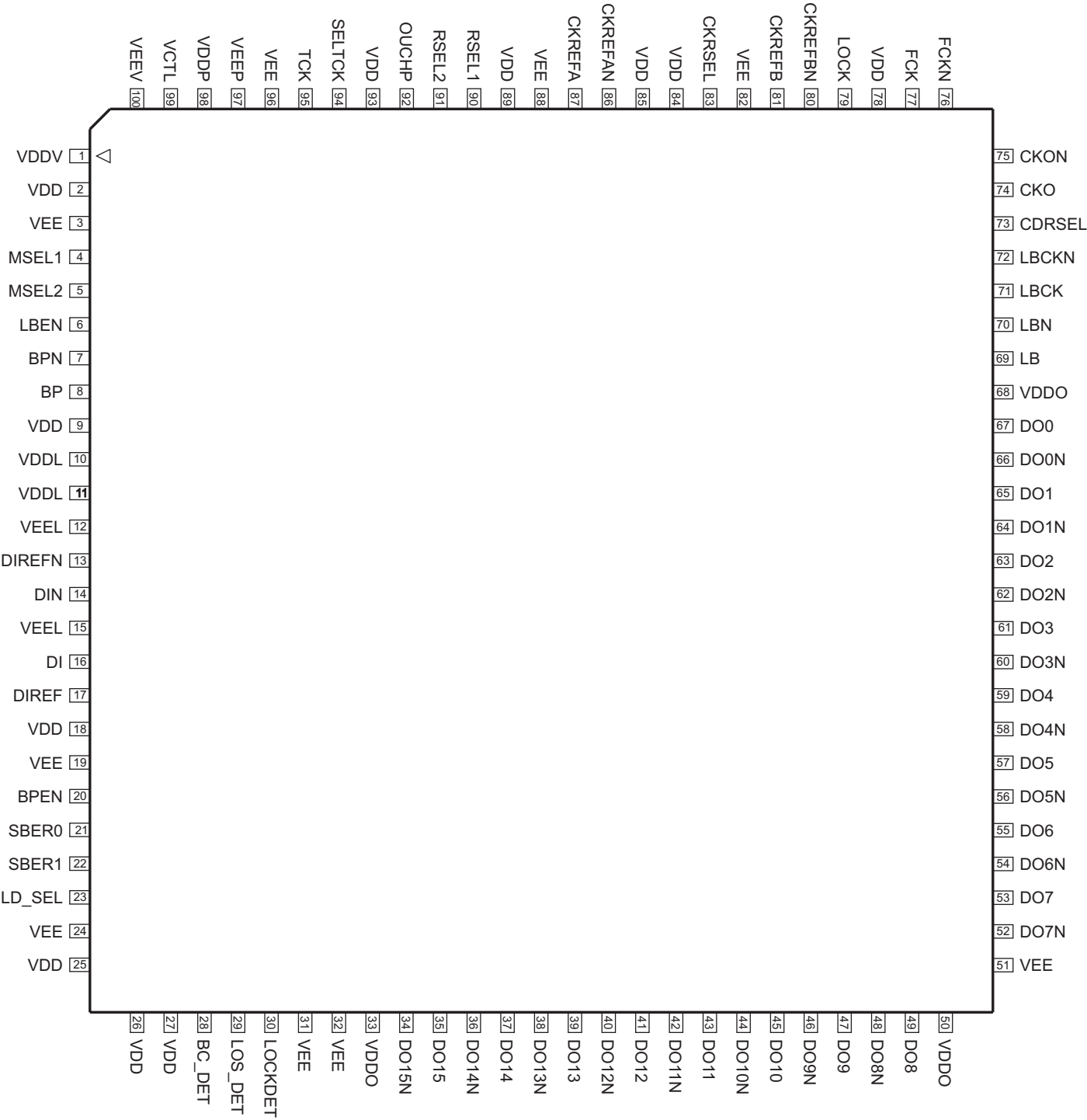
Figure 23. Package pinout, 100 pin. Top view.
