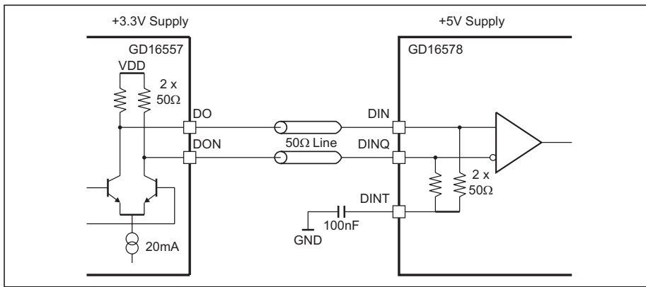
Figure 16. GD16557/GD16578 DC-connection
