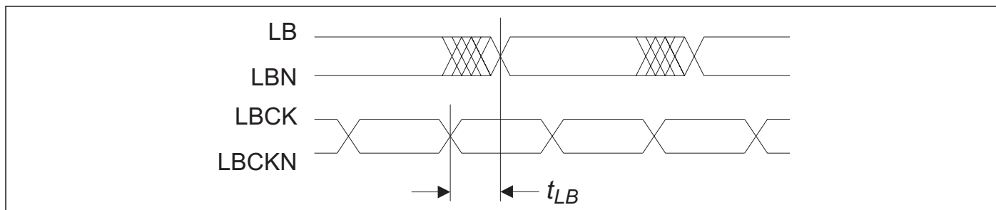
Figure 26. Loop-back Timing.
