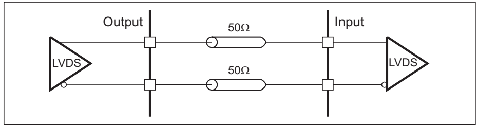
Figure 5. LVDS connection
