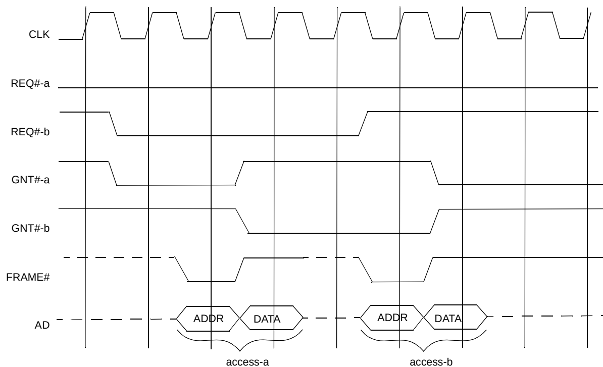
Figure 4-20. Basic Arbitration
