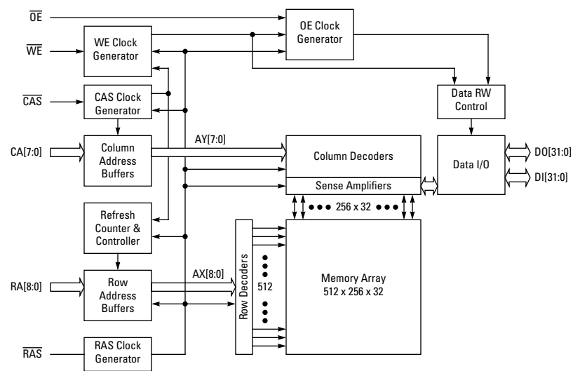
Figure 1. GLT44032-E - 128K x 32
