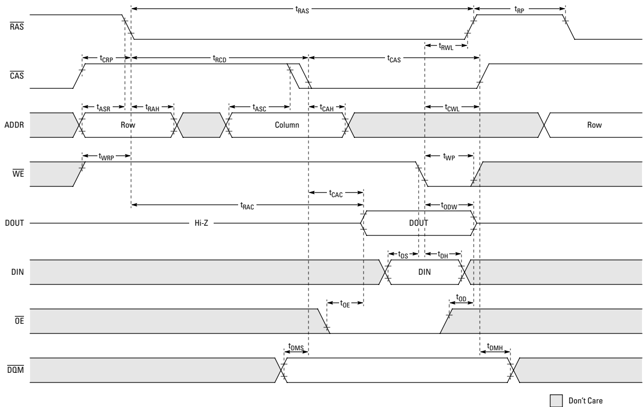
Figure 4. Read/Write Cycle
