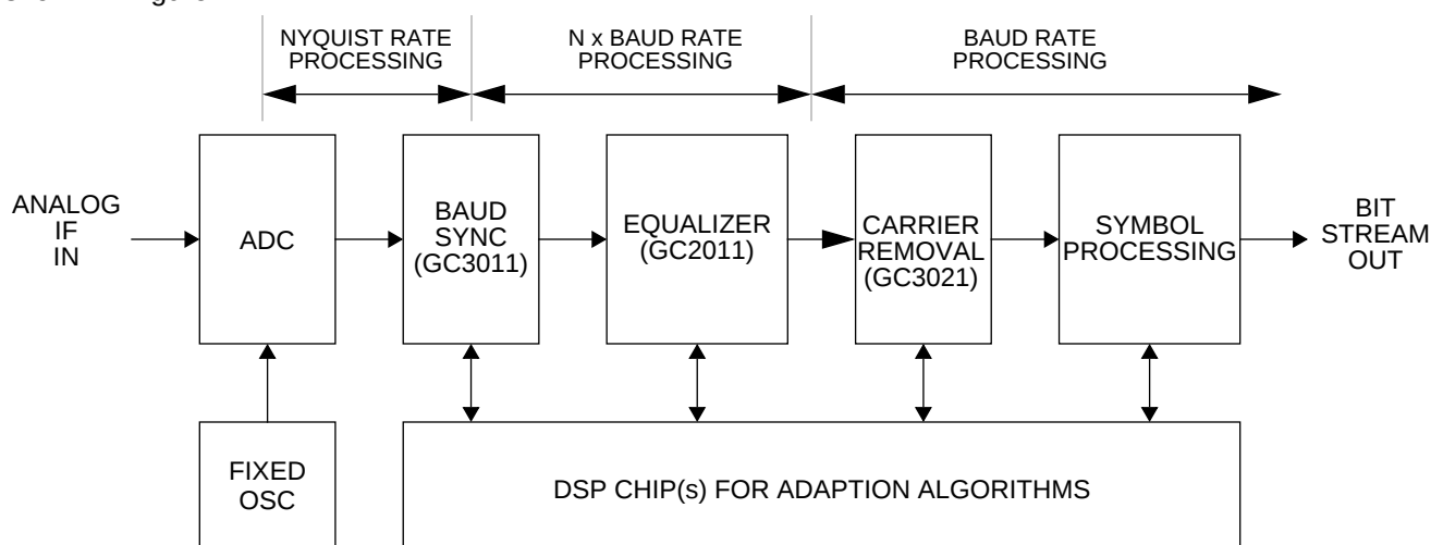
Figure 1. GENERIC DEMODULATOR
